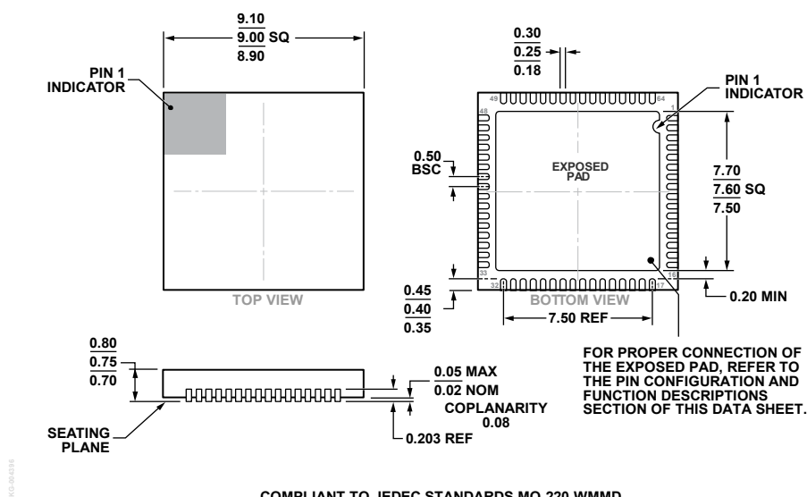
Figure 121. 64-Lead Lead Frame Chip Scale Package [LFCSP] 9 mm × 9 mm Body and 0.75 mm Package Height (CP-64-15) Dimensions shown in millimeters
