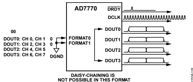
Figure 112. FORMATx Pin Configuration—FORMAT0 = 0, FORMAT1 = 0
