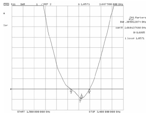
Characteristic Curves - NGAW9020S2R660GS1TRF
