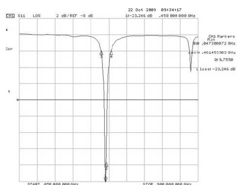
Characteristic Curves - NGAW1603S0R433GS1TRF
