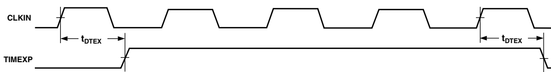
Figure 11. Timer
