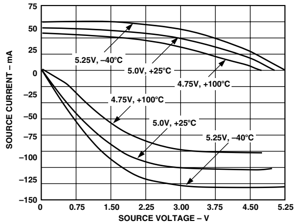
Figure 28. ADSP-2106x Typical Drive Currents ( V_{DD} = 5\text{ V} )
