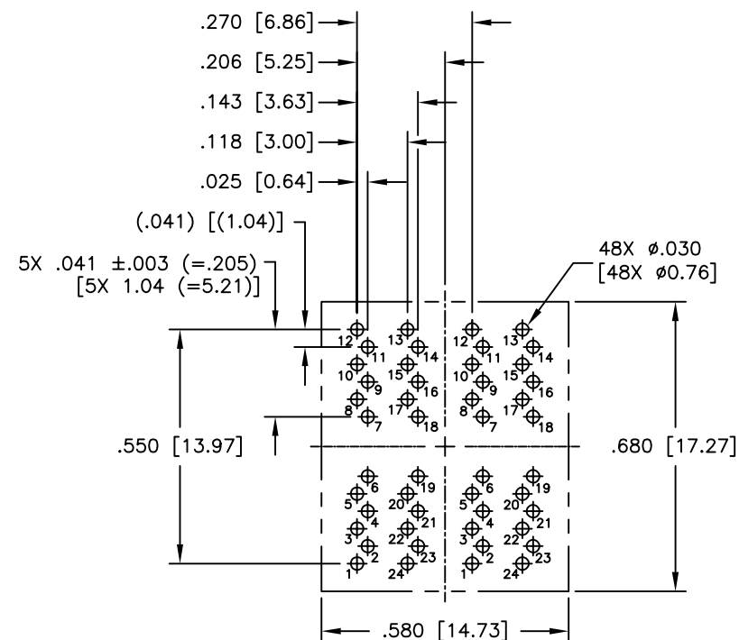
SUGGESTED PCB LAYOUT (COMPONENT SIDE SHOWN)
