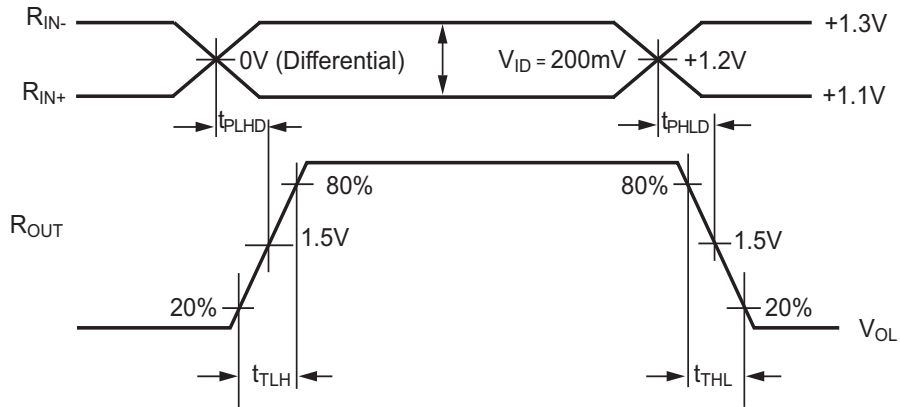
Figure 2. Receiver Propagation Delay and Transition Time Waveforms
