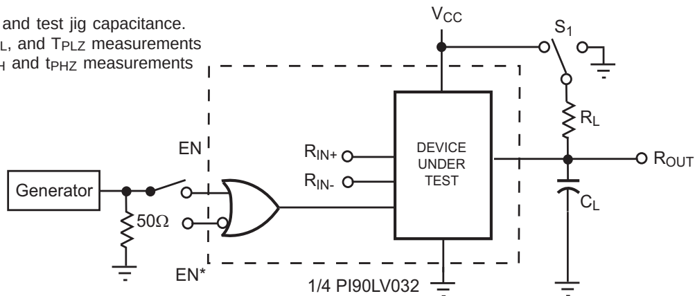
Figure 3. Receiver Three-STATE Delay Test Circuit
