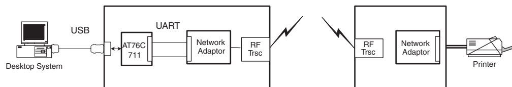
Figure 1. Typical AT76C711 Application
