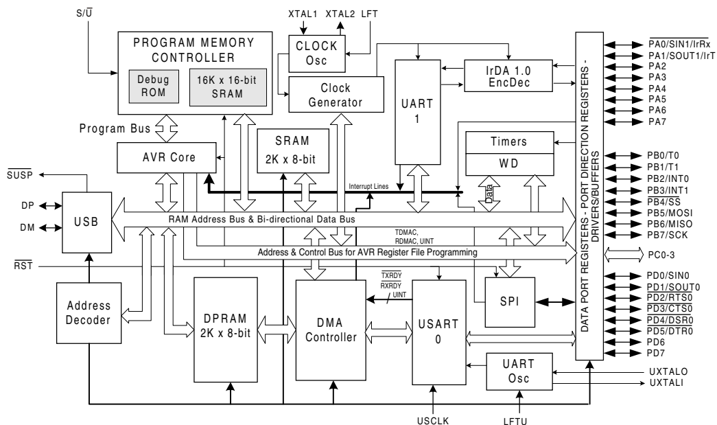
Figure 2. Functional Diagram
