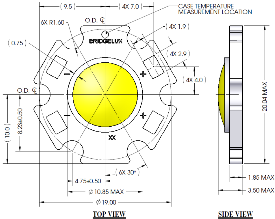
Figure 1: Drawing for 400 lumen product options (part numbers BXRA-C0402, BXRA-N0402, BXRA-W0401, BXRA-W0403, BXRA-W0402 and BXRA-C0603).
