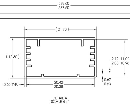
Figure 46: Tube Design for Hexagonal Star Products
