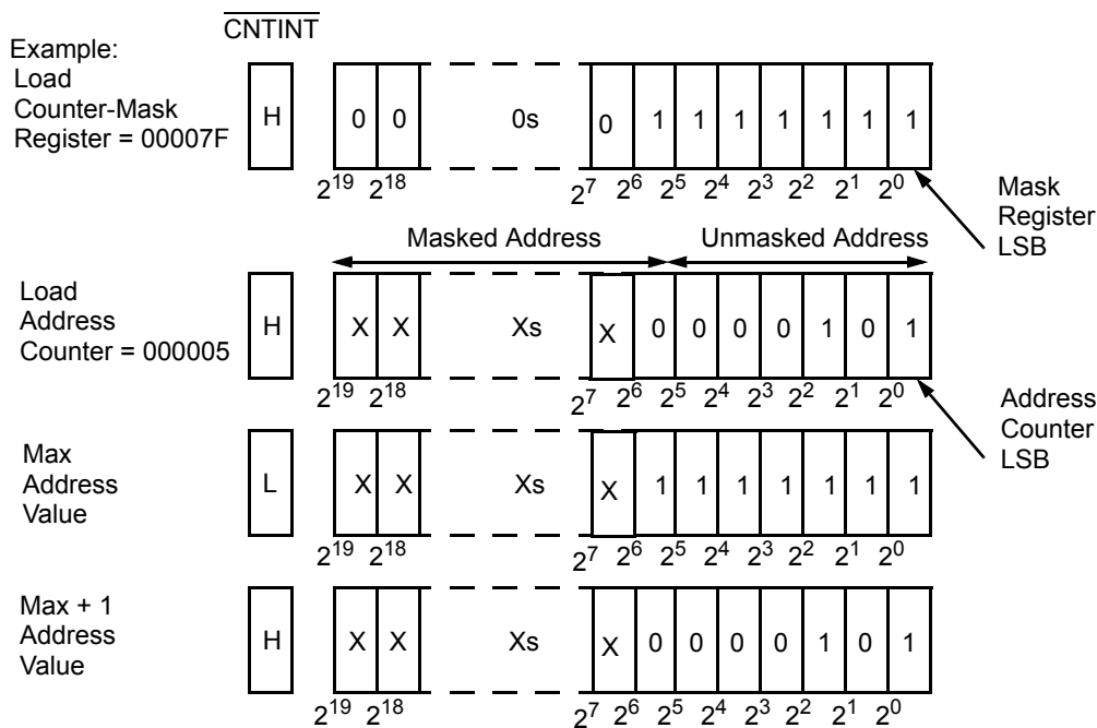
Figure 5. Programmable Counter-Mask Register Operation with WRP deasserted [1,25]
