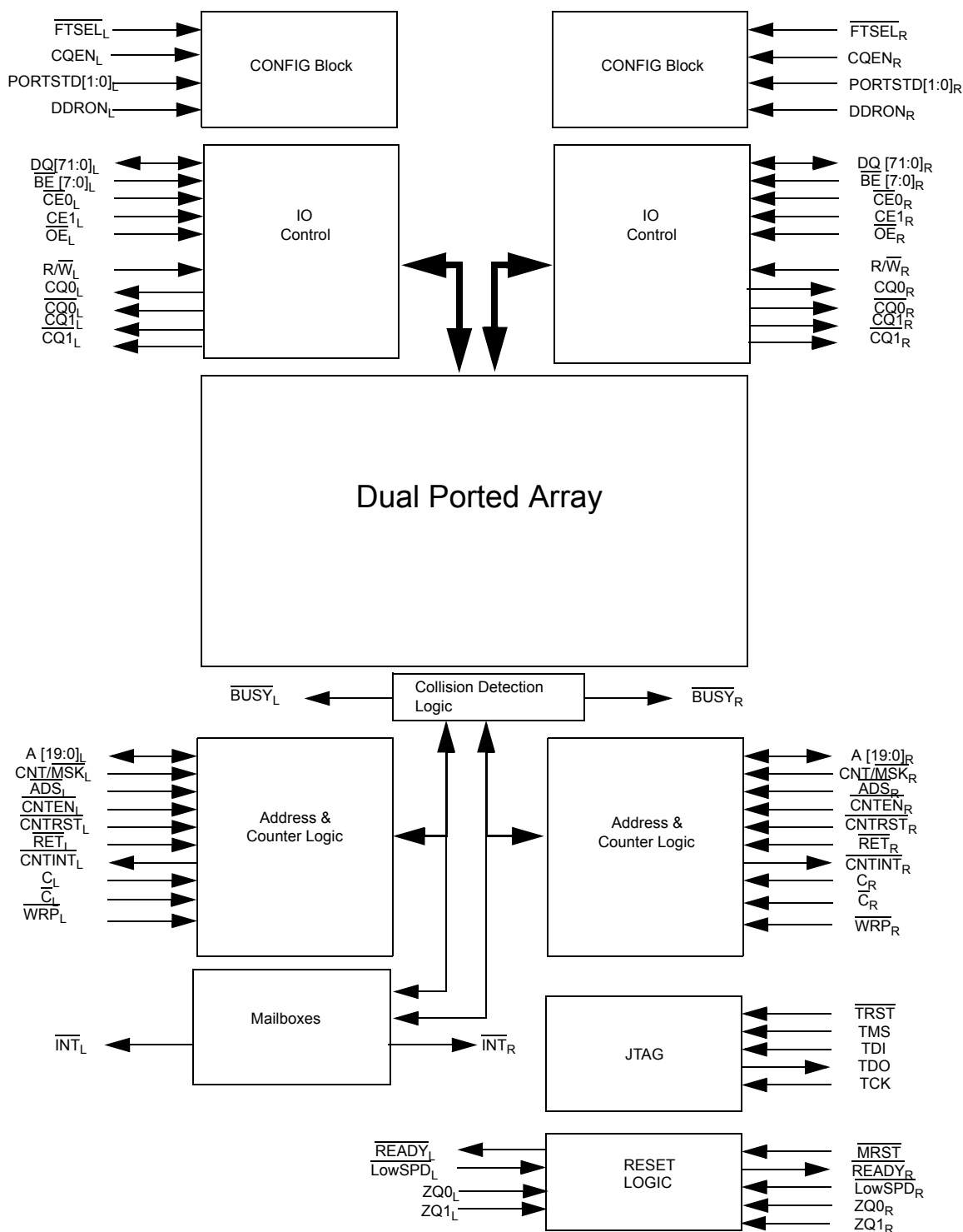
Figure 1. Block Diagram [1,2,3]
