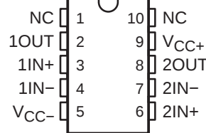
TLE2142 U PACKAGE (TOP VIEW)
