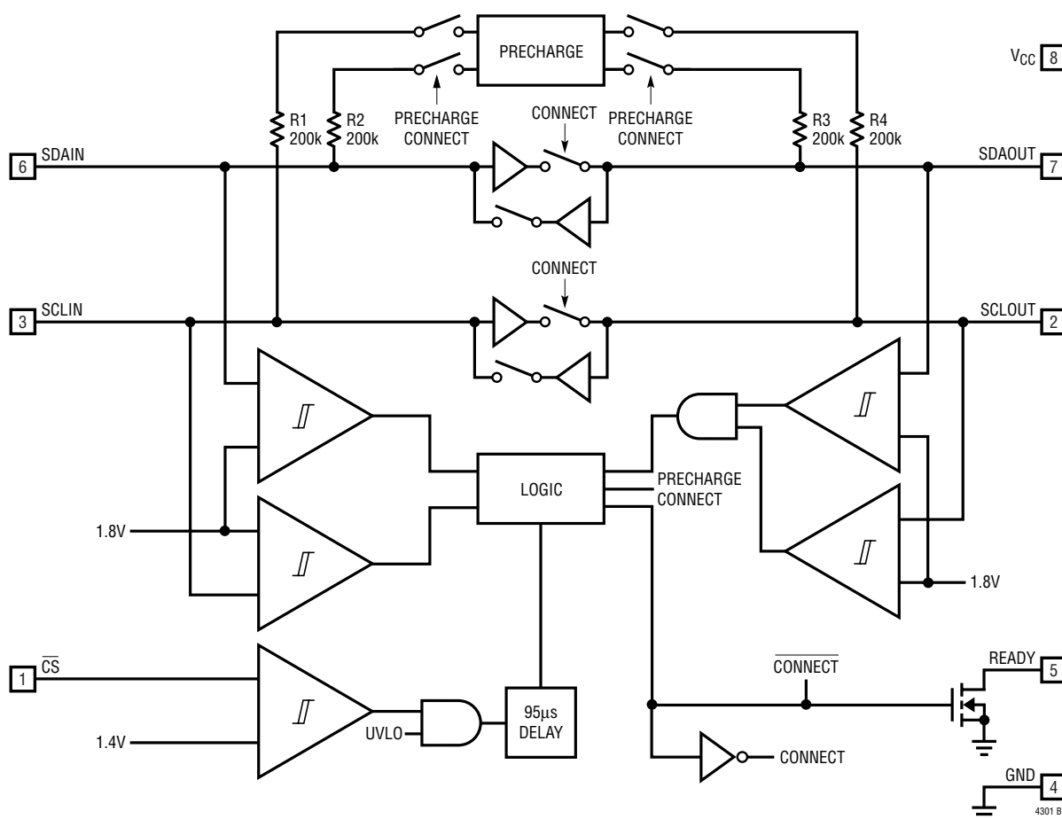
LTC4301 Supply Independent 2-Wire Bus Buffer
