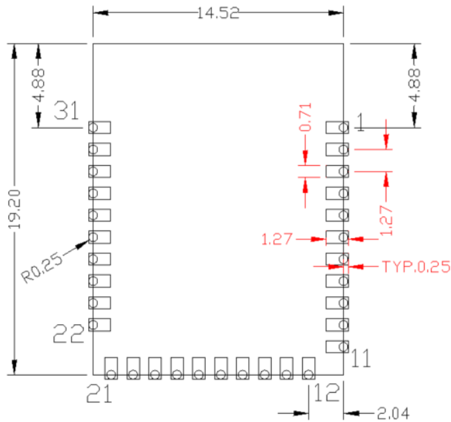
Figure 4. Host Layout Pattern for CYBLE-2120XX-X0
