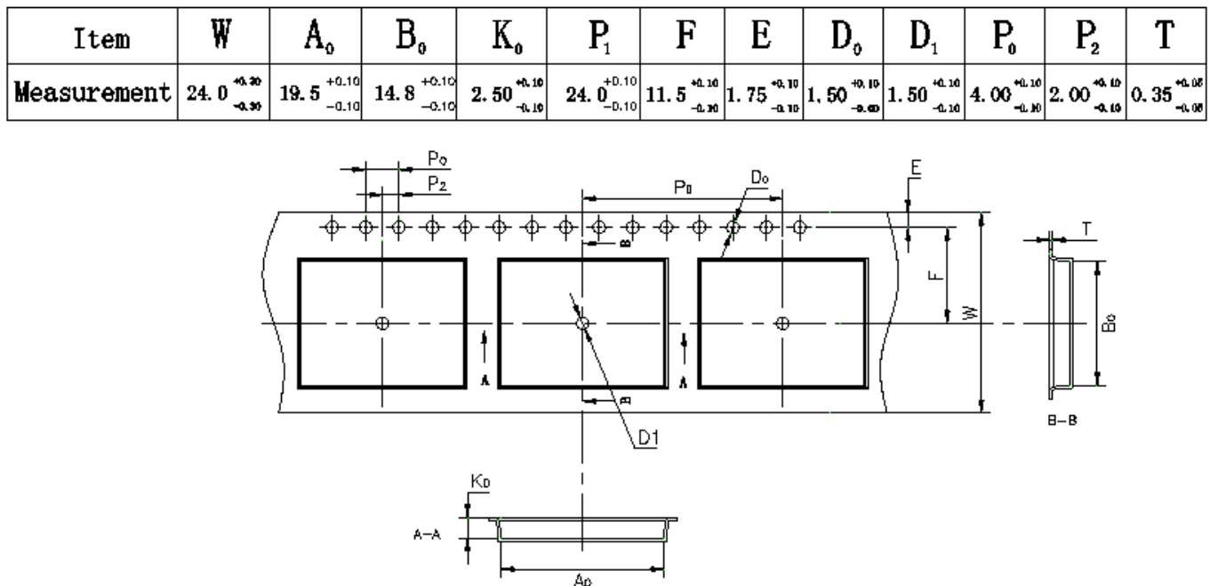
Figure 10. CYBLE-2120XX-X0 Tape Dimensions
