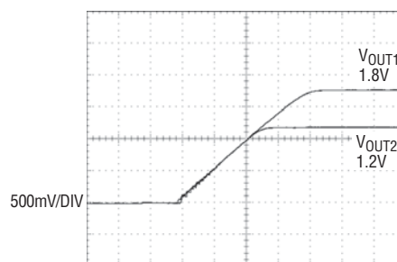
Tracking Start-Up with Internal Soft-Start ( C_{RUN/SS} = 0\mu\text{F} )
