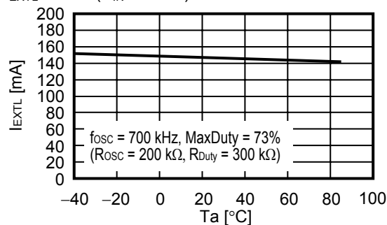
I_{EXTL} vs. T_a ( V_{IN} = 3.3\text{ V} )
