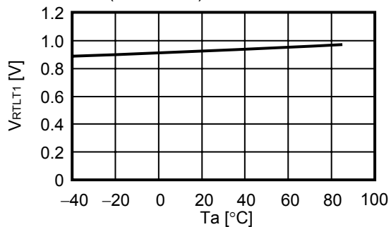
V_{RTLT1} vs. T_a ( V_{IN} = 3.3 V)
