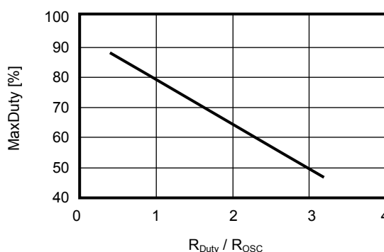
Figure 13 RDuty / ROSC vs. MaxDuty
