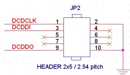
<Fig.3.3> W7100 Debugger Connector
