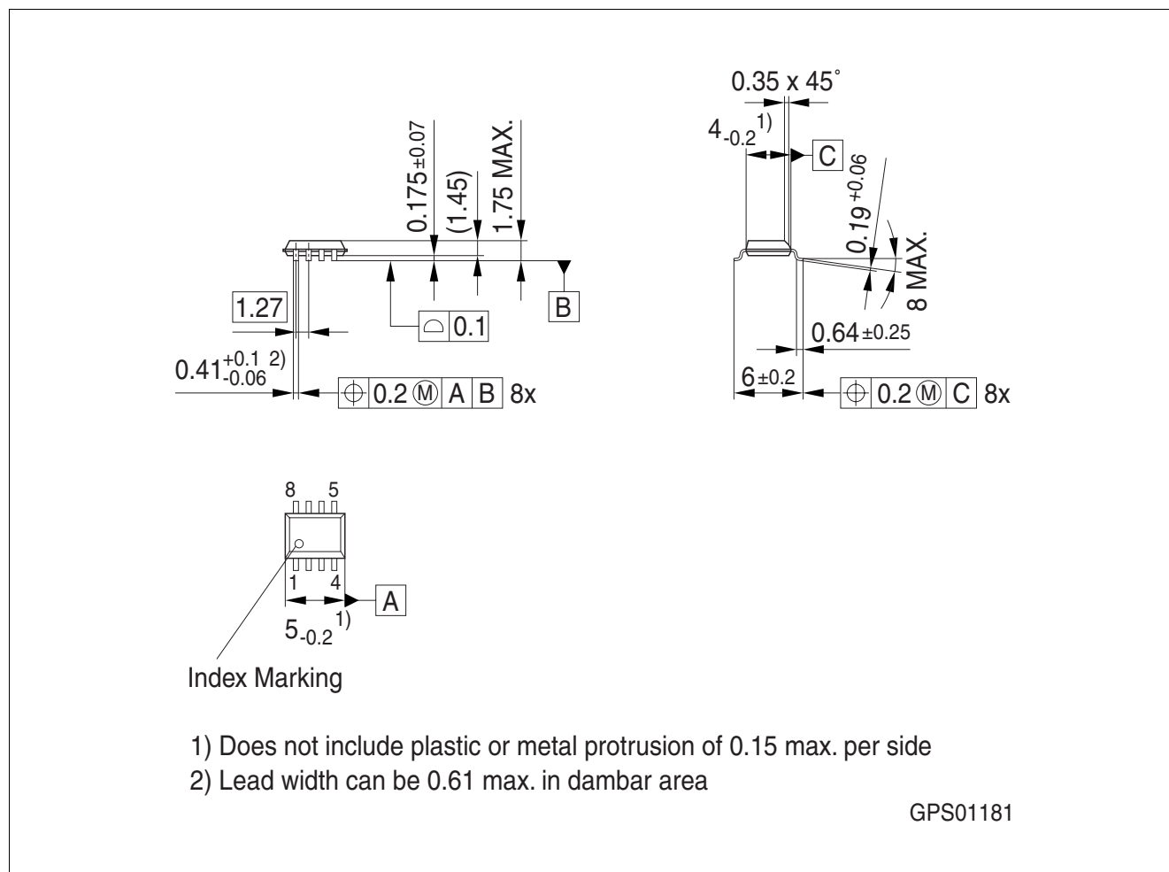
Figure 9 PG-DSO-8
