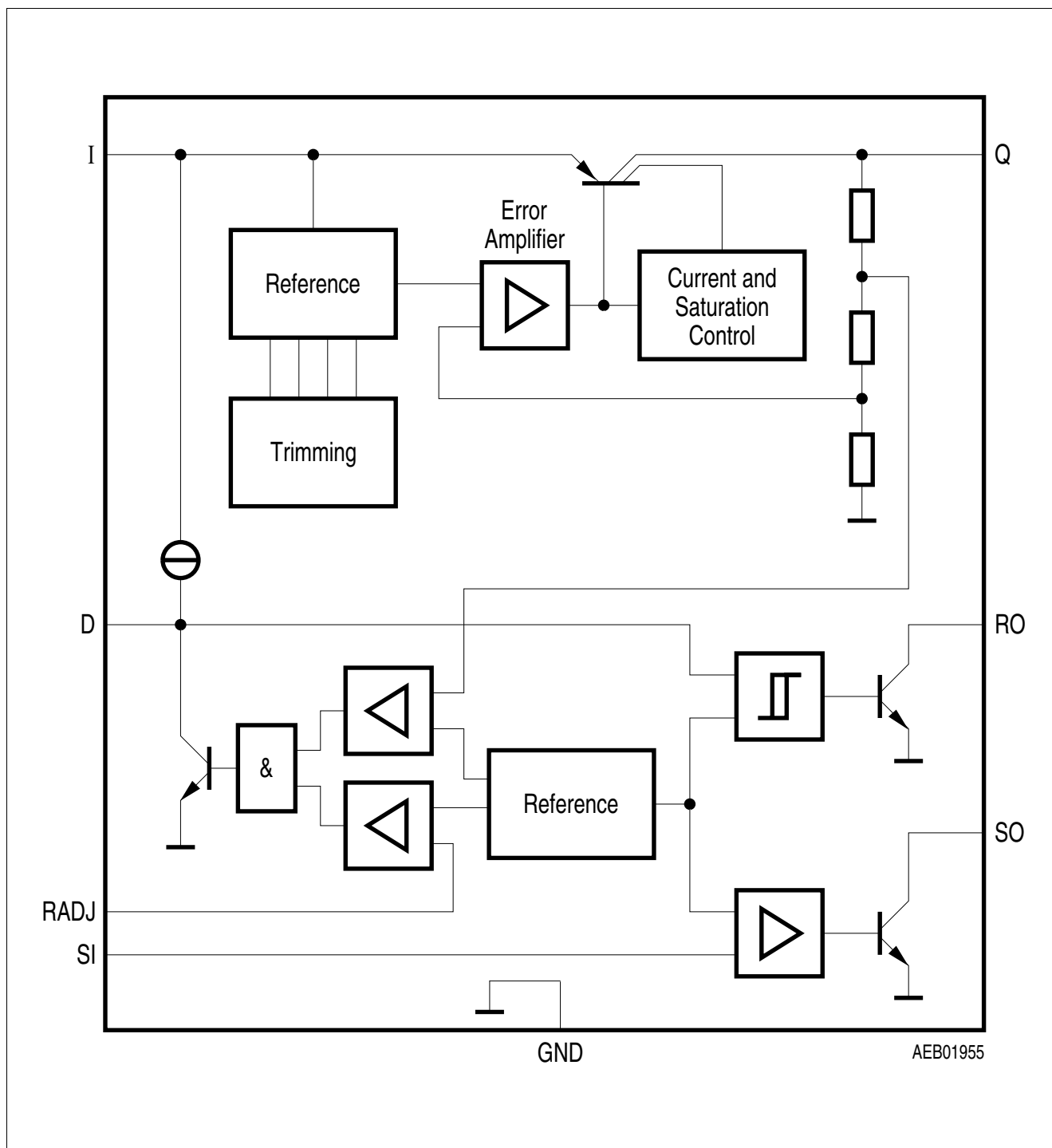
Figure 1 Block Diagram
