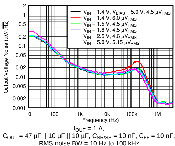
Figure 5. Output Voltage Noise vs Frequency and V_{IN}
