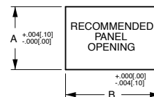
TERMINAL TYPE
