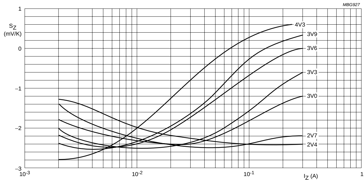
BZV90-C2V4 to C4V3. T_j = 25 to 150 °C.
