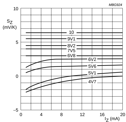
BZV90-C4V7 to C10. T_j = 25 to 150 °C.
