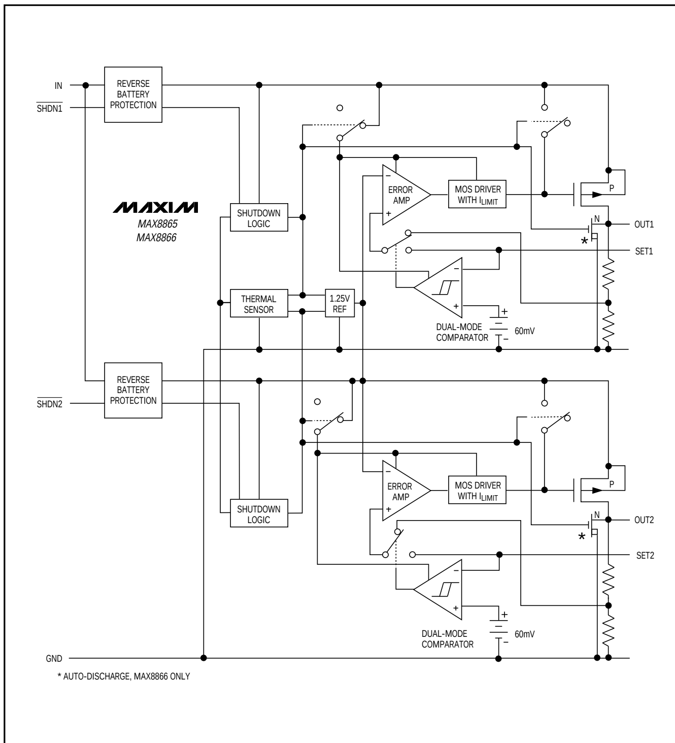
Figure 1. Functional Diagram
