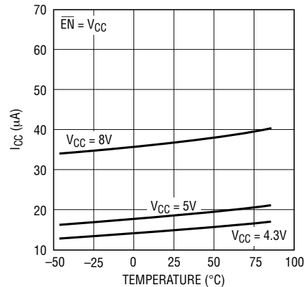
Shutdown Supply Current vs Temperature and V_{\text{CC}}
