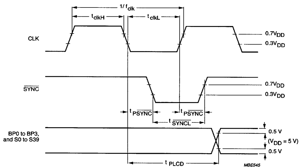
Fig.21 Driver timing waveforms.
