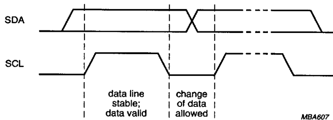
Fig.12 Bit transfer.
