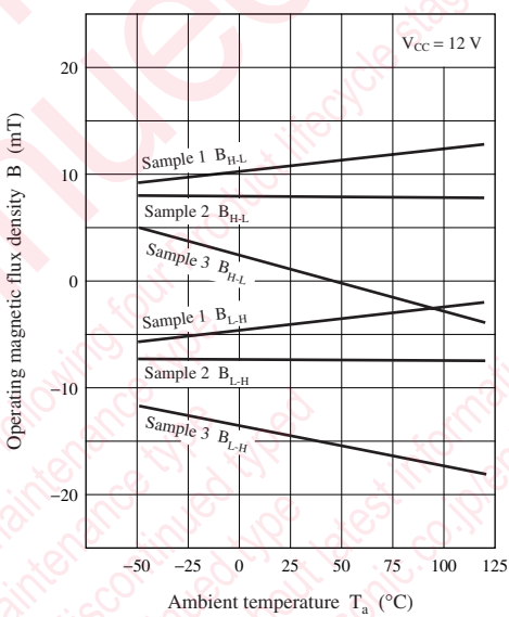
Operating magnetic flux density — Ambient temperature
