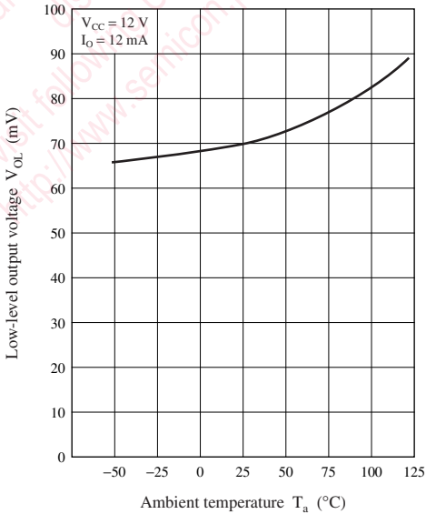
Low-level output voltage — Ambient temperature
