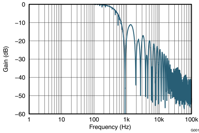
Figure 6-1. Frequency Response
