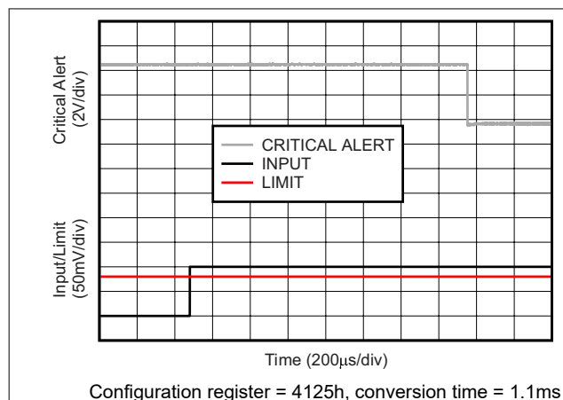
Figure 8-2. Critical Alert Response for 1.1ms Conversion Time
