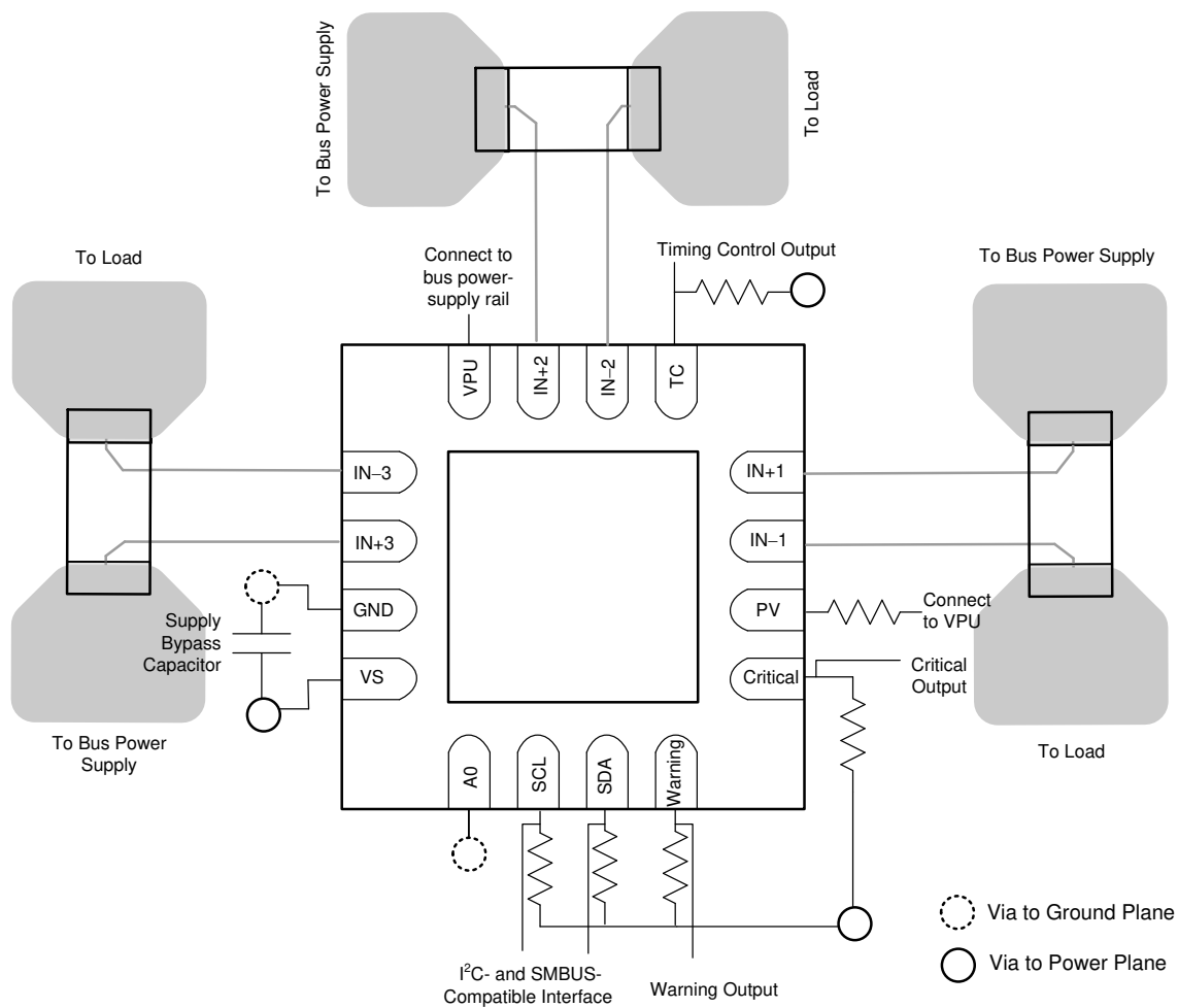
Figure 8-4. Layout Example
