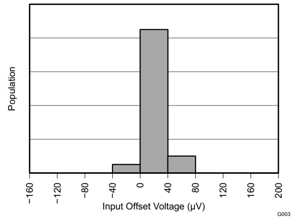
Figure 6-2. Shunt Input Offset Voltage Production Distribution
