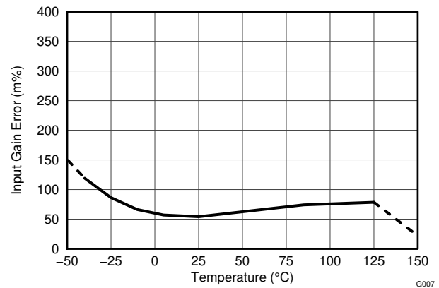
Figure 6-6. Shunt Input Gain Error vs. Temperature
