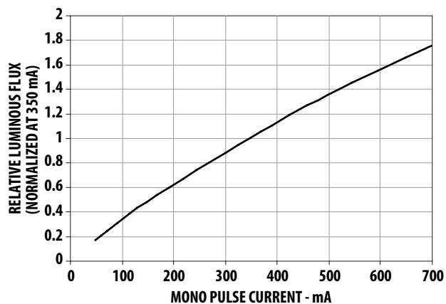
Figure 4. Relative Luminous Flux vs. Mono Pulse Current
