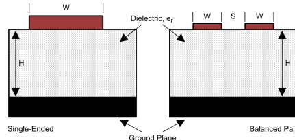
Figure 36. Microstrip Topology
