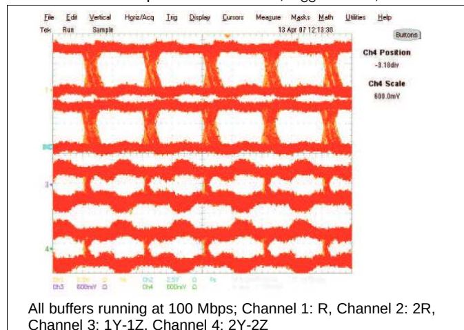
Figure 30. Typical Eye Pattern SN65LVDS050: All Buffers
