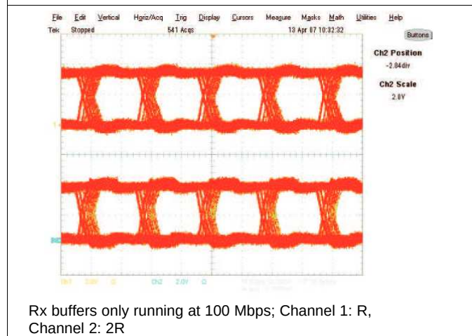
Figure 34. Typical Eye Pattern SN65LVDS051: Rx Buffers
