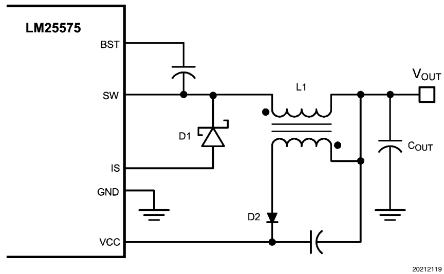
FIGURE 12. VCC Bias with Additional Winding on the Output Inductor
