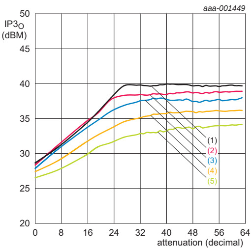
V_{SUP} = 5\text{ V} ; T_{amb} = 25\text{ °C} . (1) f = 0.4\text{ GHz} (2) f = 0.7\text{ GHz} (3) f = 1.45\text{ GHz} (4) f = 2.10\text{ GHz} (5) f = 2.75\text{ GHz}
