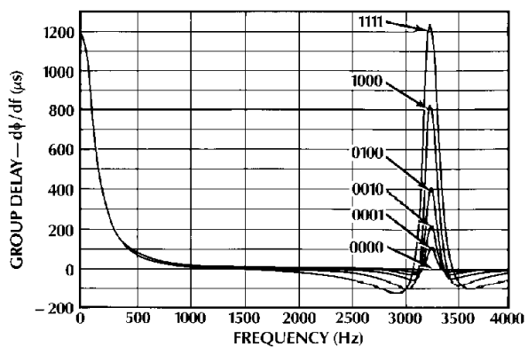
Figure 4. Typical Height Filter Response — NL/L = 0
