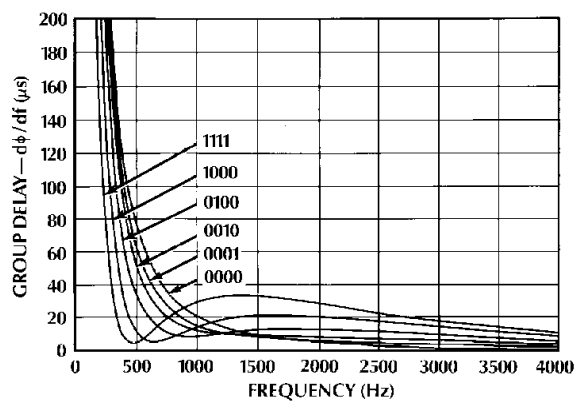
Figure 3. Typical Slope Filter Response — NL/L = 1
