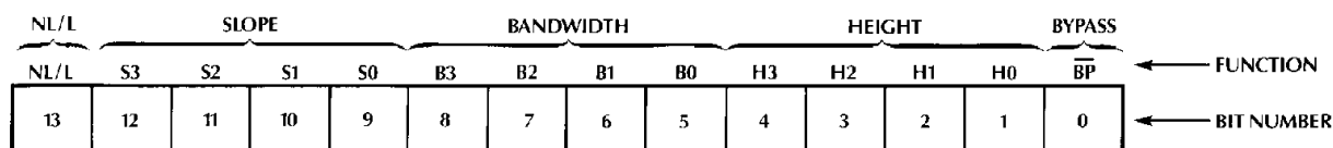
Figure 7. 14-Bit Latch
