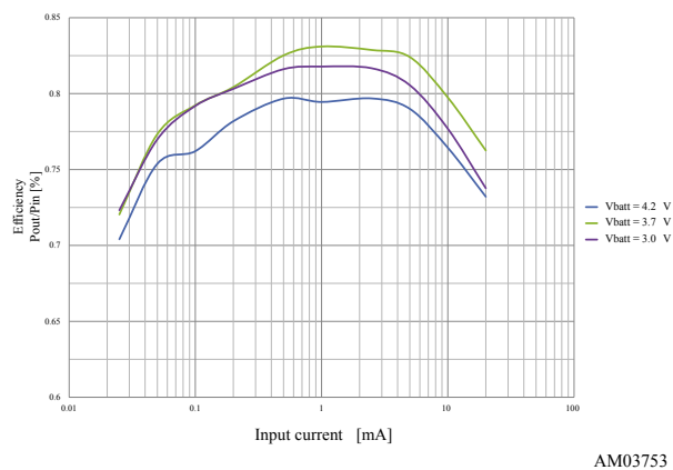
Figure 19. Efficiency vs. input current - V_{OC} = 15V
