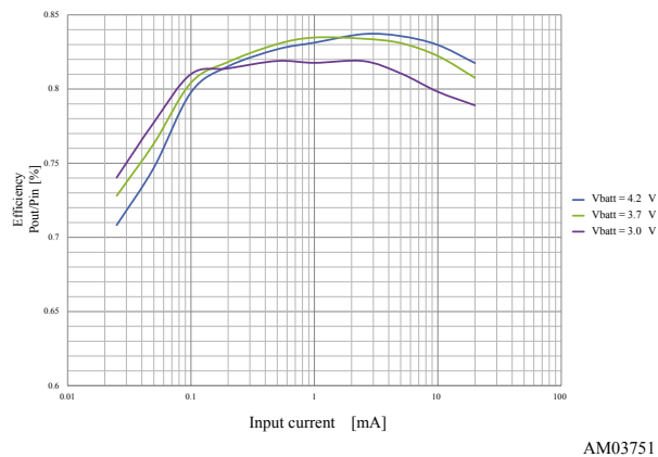
Figure 17. Efficiency vs. input current - V_{OC} = 9V
