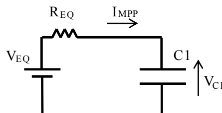
Figure 21. Energy harvester equivalent circuit
