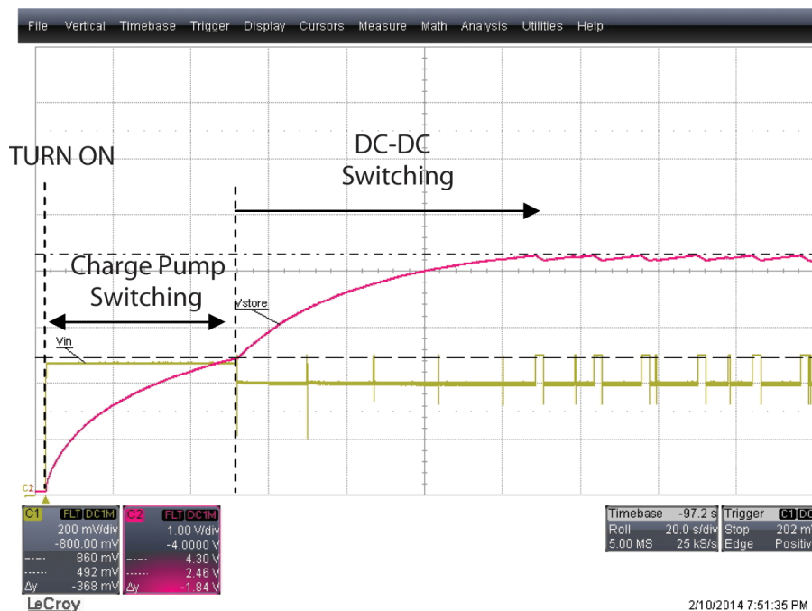
Figure 6. Boost start-up
