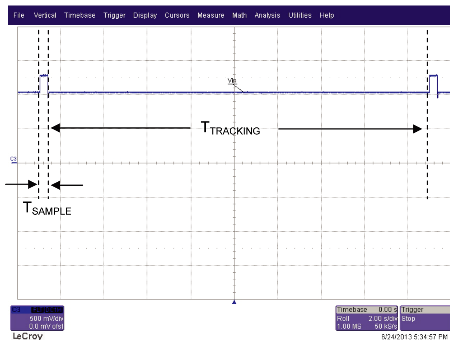
Figure 7. MPPT tracking
