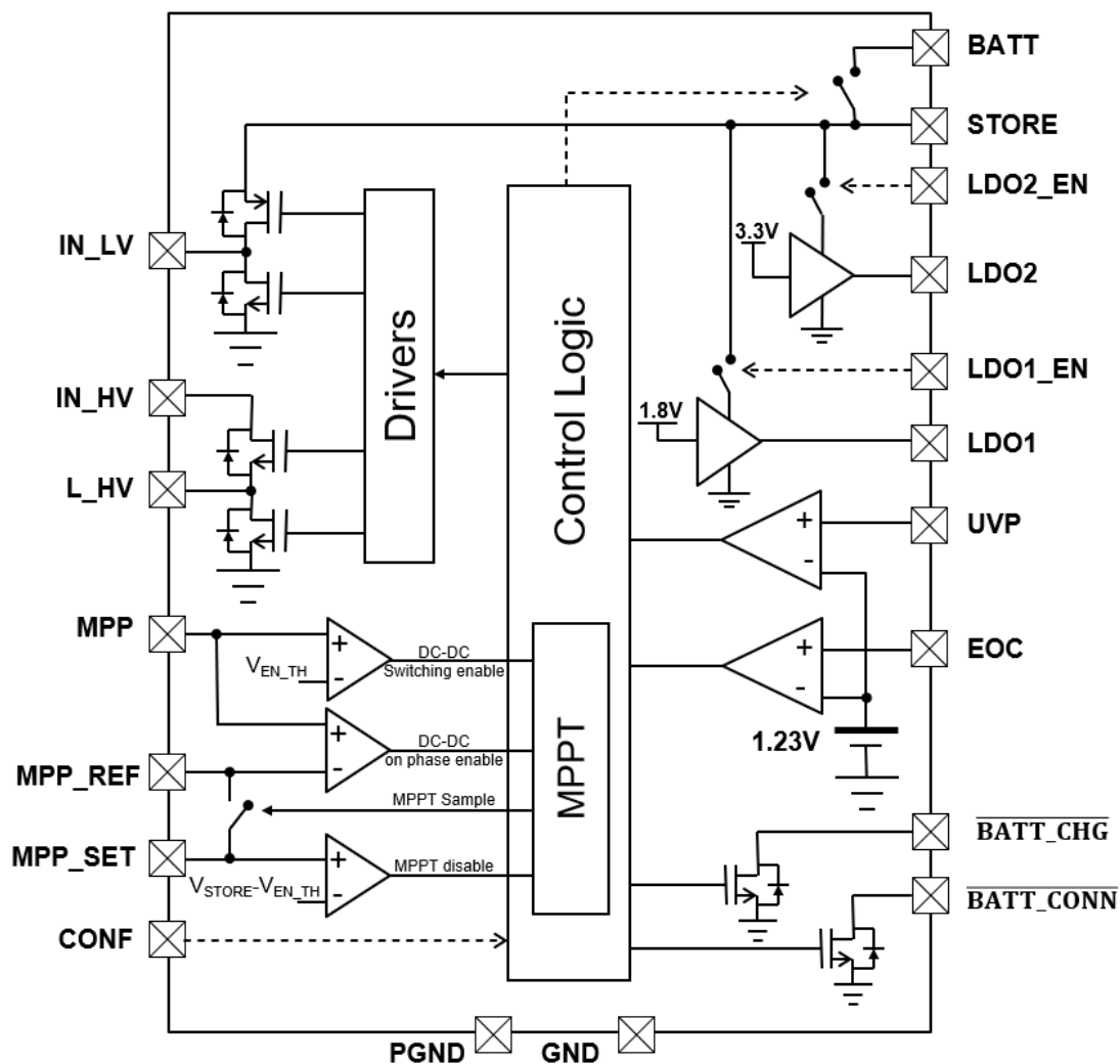
Figure 1. Block diagram
