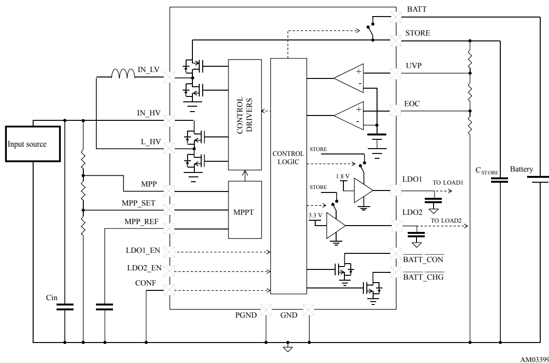
Figure 13. Buck-boost configuration example
