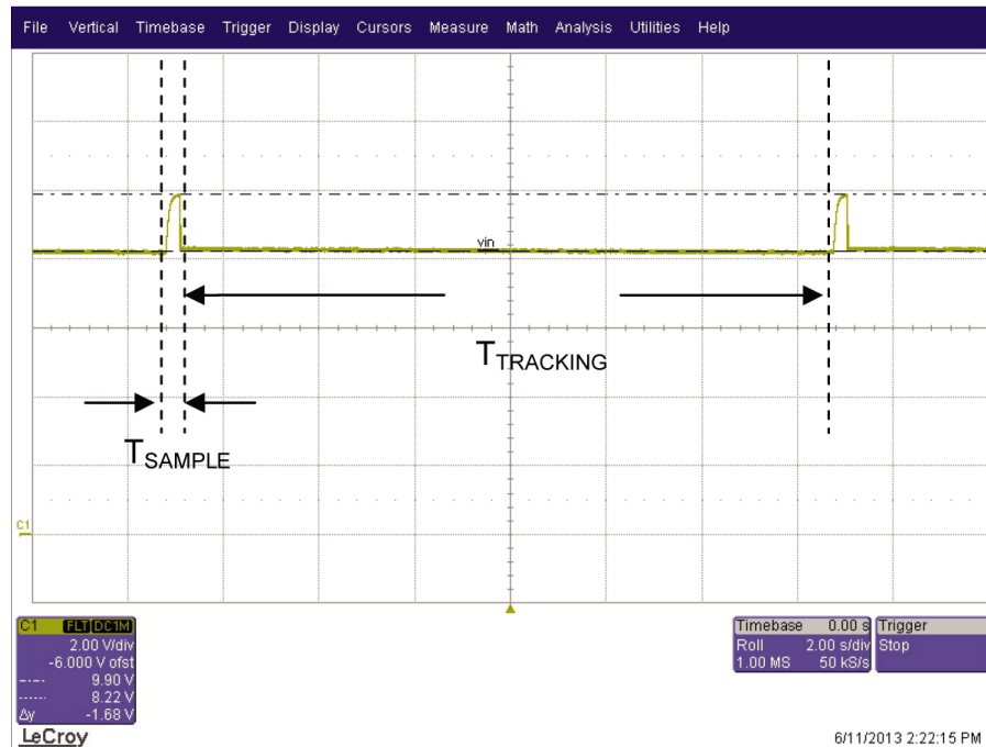
Figure 15. MPPT tracking
