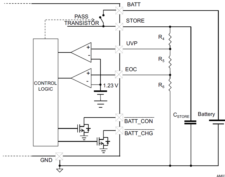
Figure 3. Battery management section
