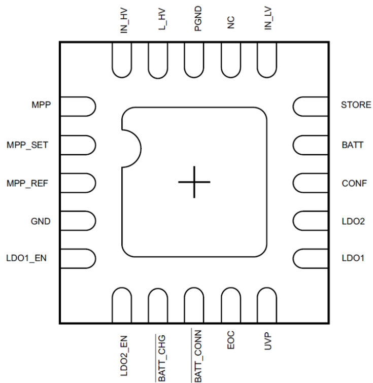
Figure 2. Pin configurations
