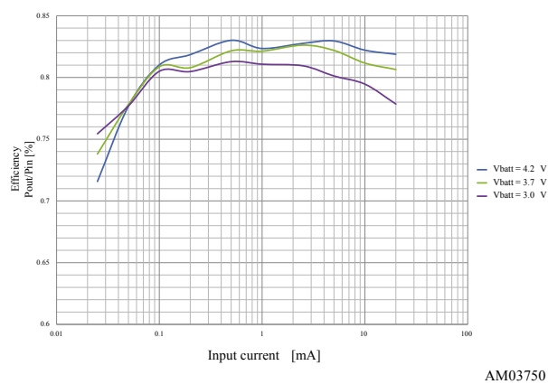
Figure 16. Efficiency vs. input current - V_{OC} = 6V
