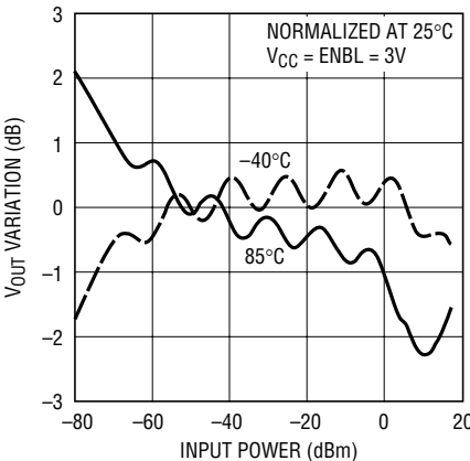
V OUT Variation vs Input Power at 10MHz
