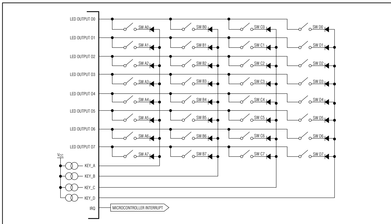
Figure 11. Key-Scanning Configuration
