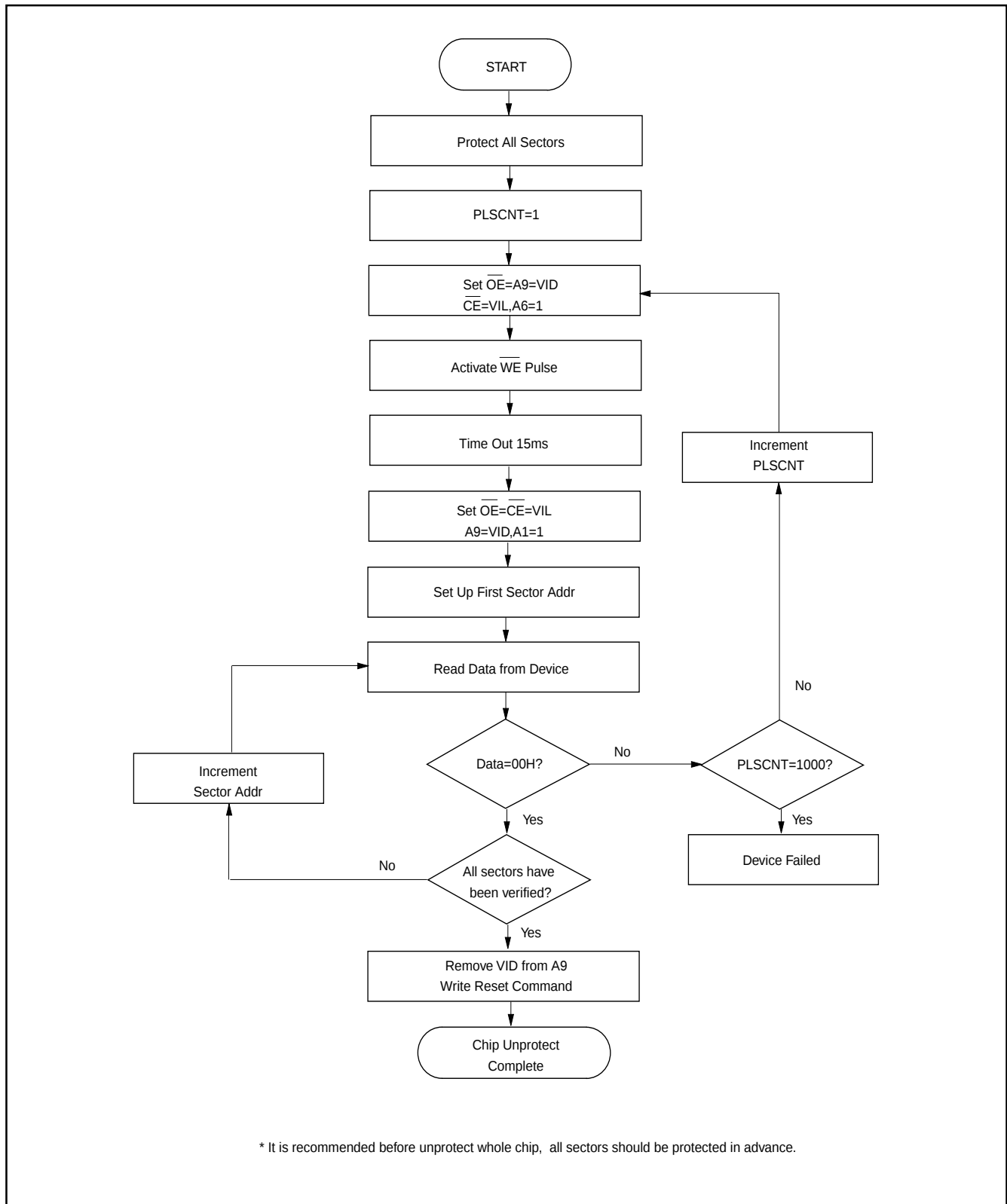
Fig 17. CHIP UNPROTECTED FLOWCHART(A9, OE Control)
