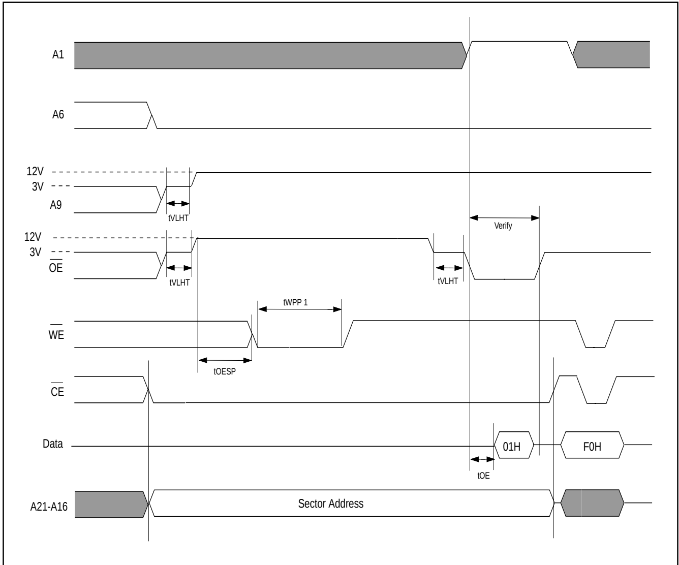
Fig 14. SECTOR GROUP PROTECT TIMING WAVEFORM (A9, \overline{\text{OE}} Control)
