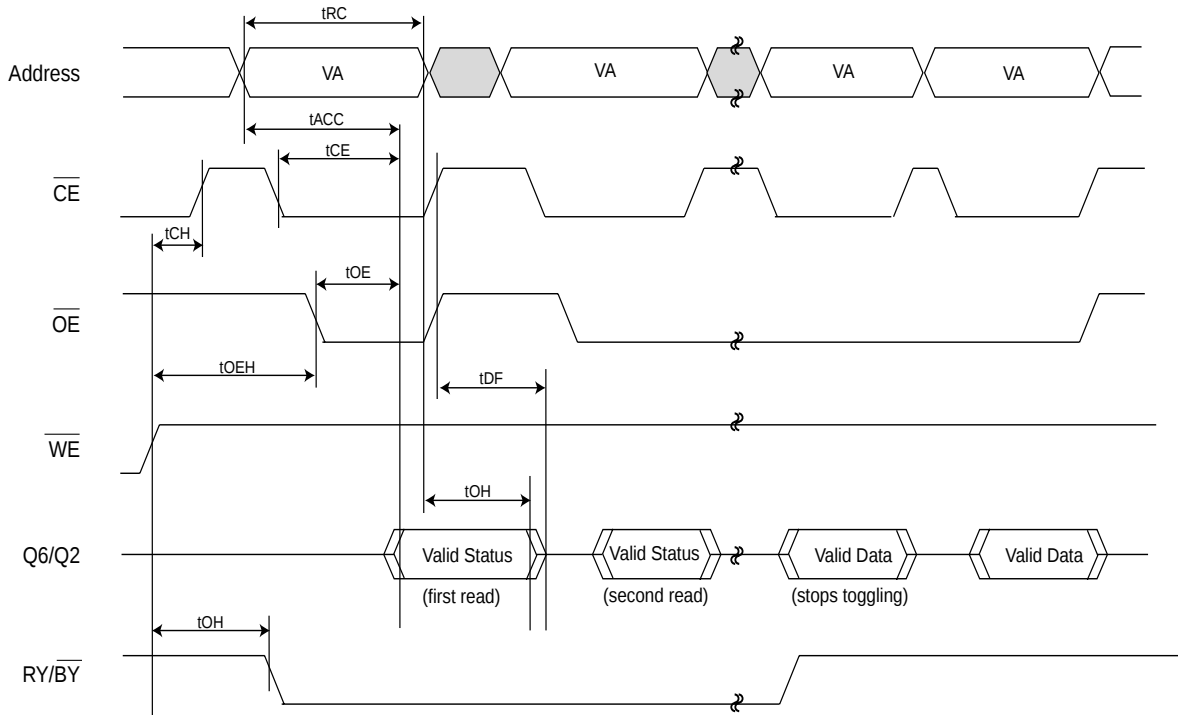
Fig 24. TOGGLE BIT TIMING WAVEFORMS (DURING AUTOMATIC ALGORITHMS)
