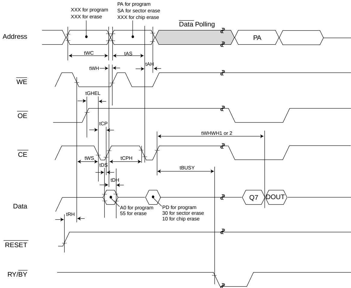
Fig 11. CE CONTROLLED PROGRAM TIMING WAVEFORM
