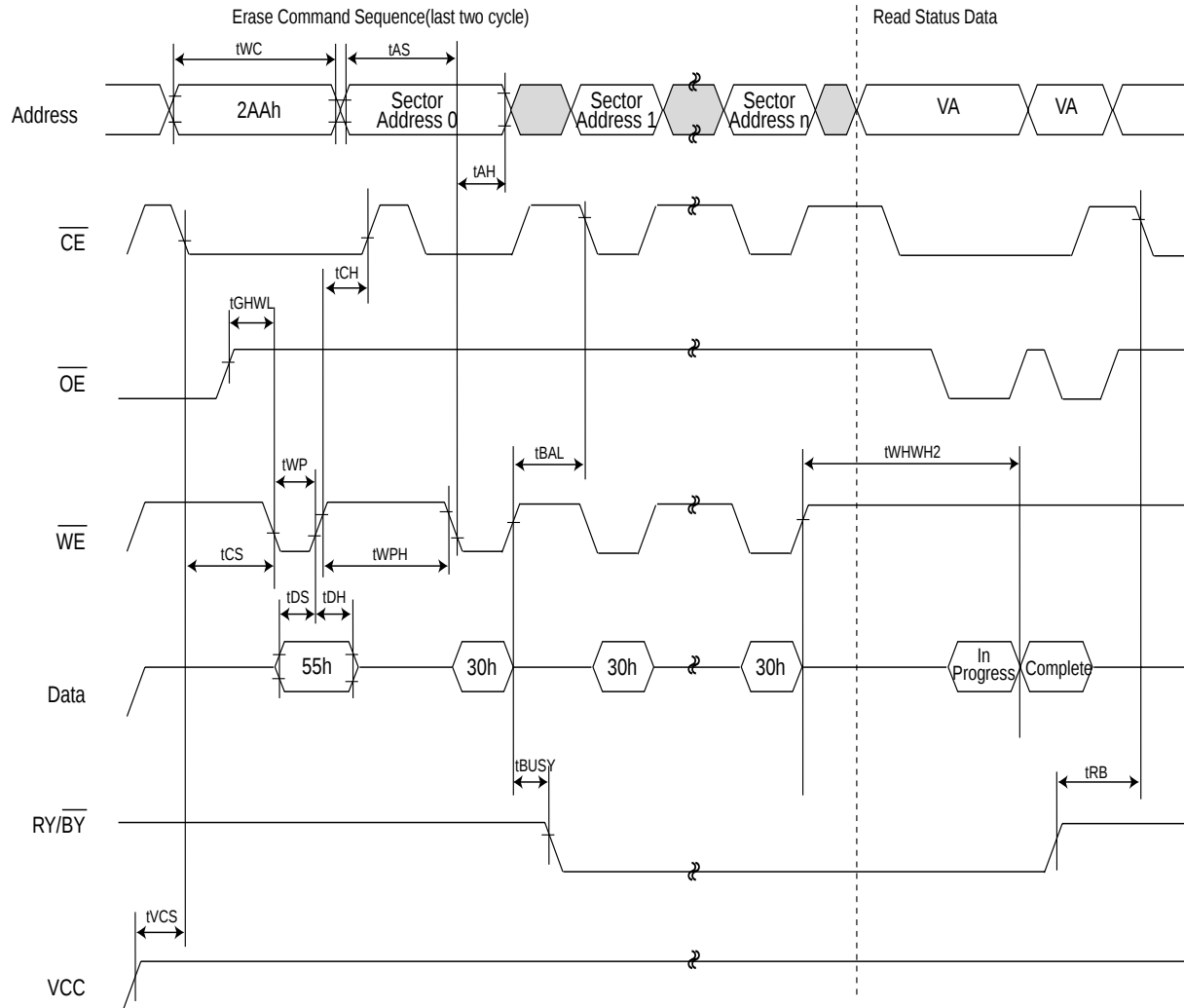
Fig 6. AUTOMATIC SECTOR ERASE TIMING WAVEFORM
