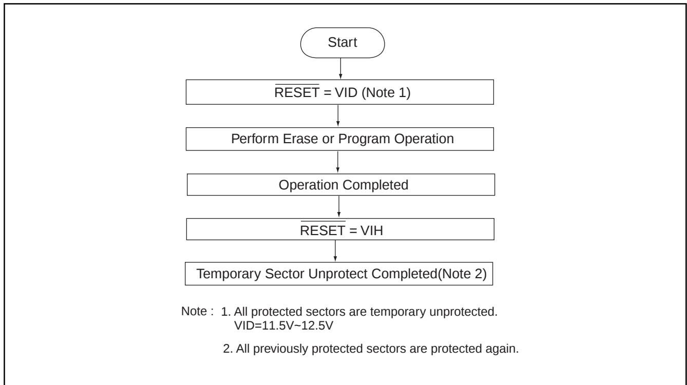
Fig 20. TEMPORARY SECTOR GROUP UNPROTECTED FLOWCHART
