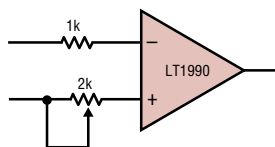
Figure 1. Optional CMRR Trim
