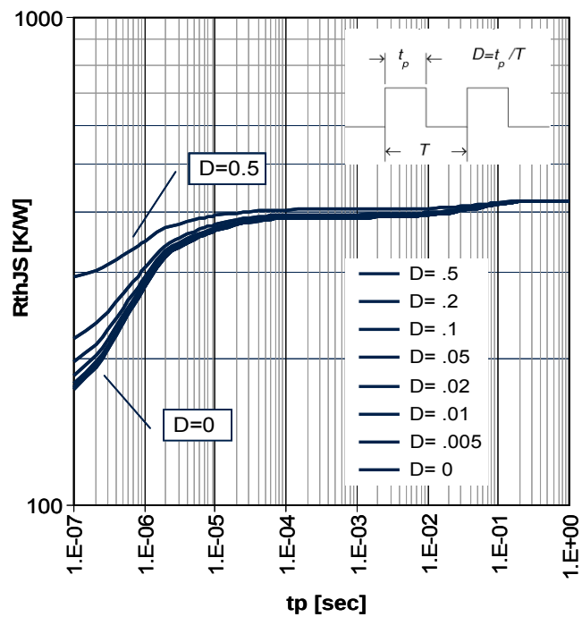
Figure 4-3 Permissible Pulse Load R_{\text{thJS}} = f(t_p)
