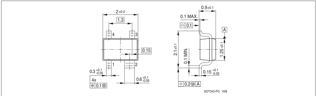
Figure 7-1 Package Outline
