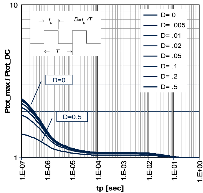
Figure 4-2 Permissible Pulse Load P_{\text{tot\_max}} / P_{\text{tot\_DC}} = f(t_p)
