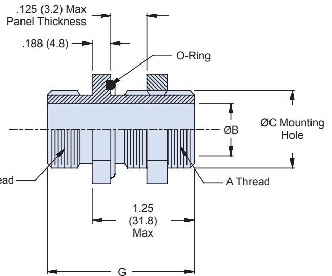
Bulkhead Feed-Throughs 710-102/103/373
