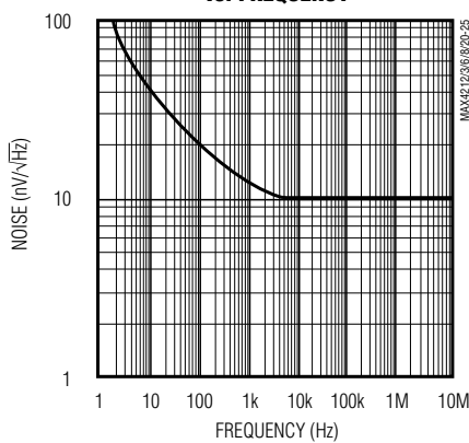
MAX4213 VOLTAGE-NOISE DENSITY vs. FREQUENCY
