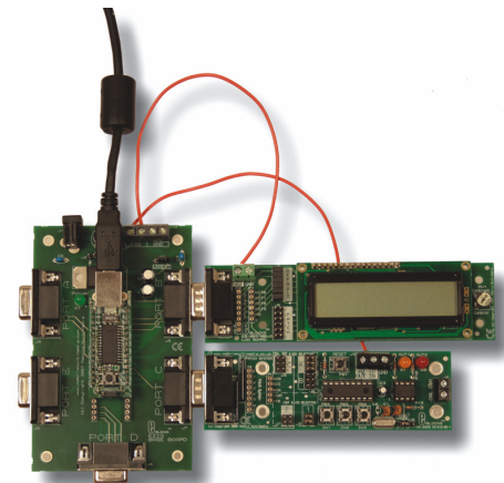
Using ECIO with E-blocks
