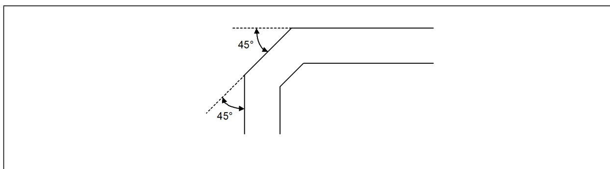
Figure 12-15. Trace Routing
