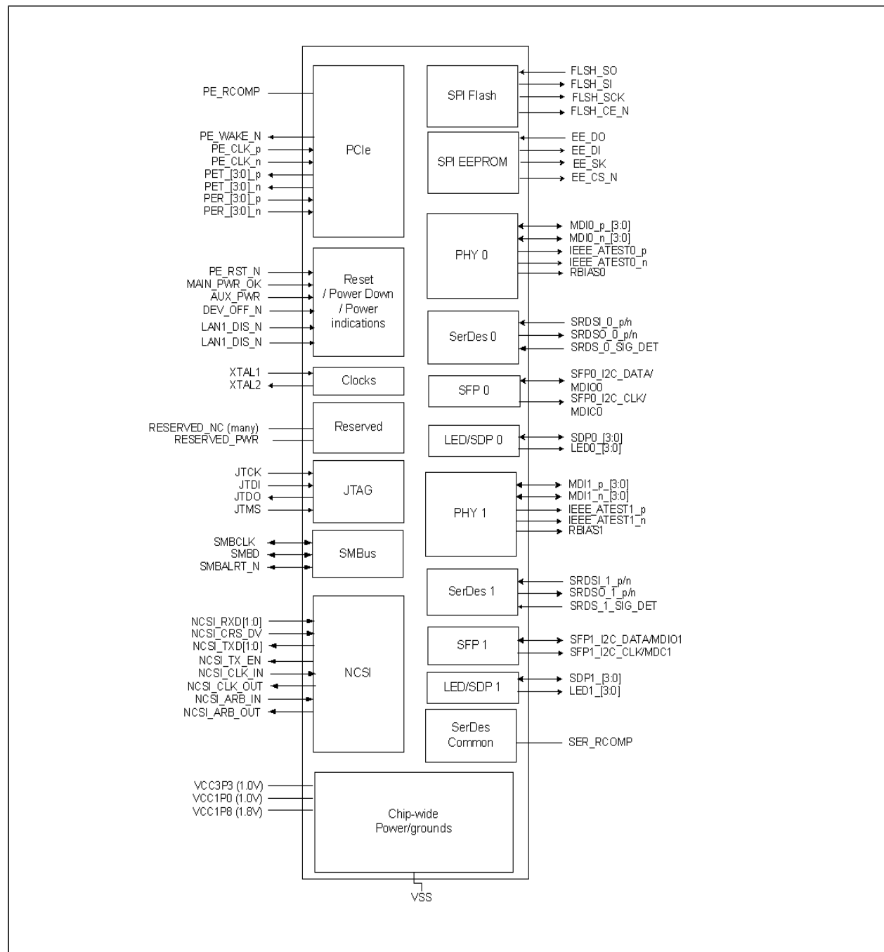
Figure 2-1. 82576 Interface Diagram
