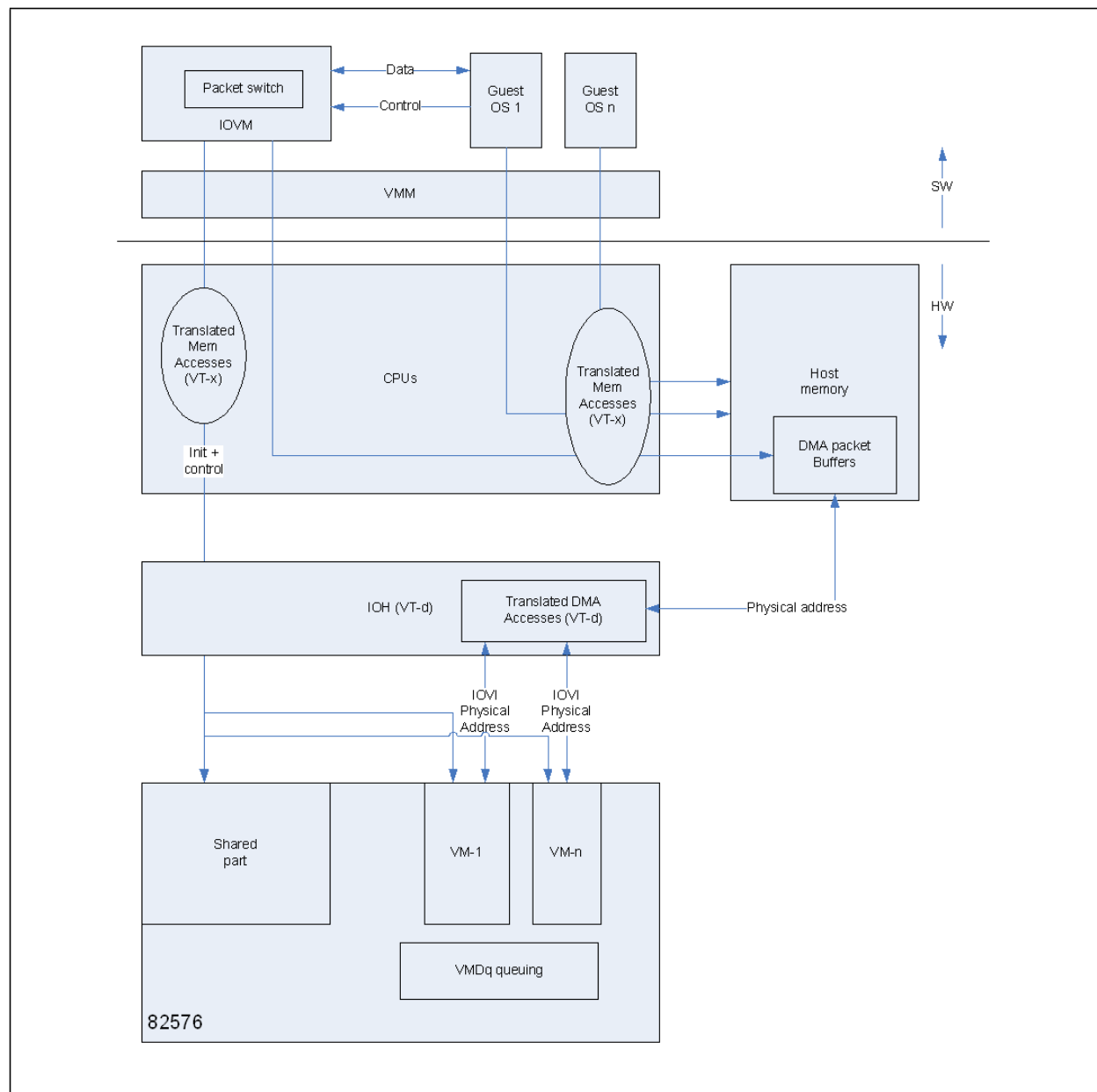
Figure 7-25. IOVM System
