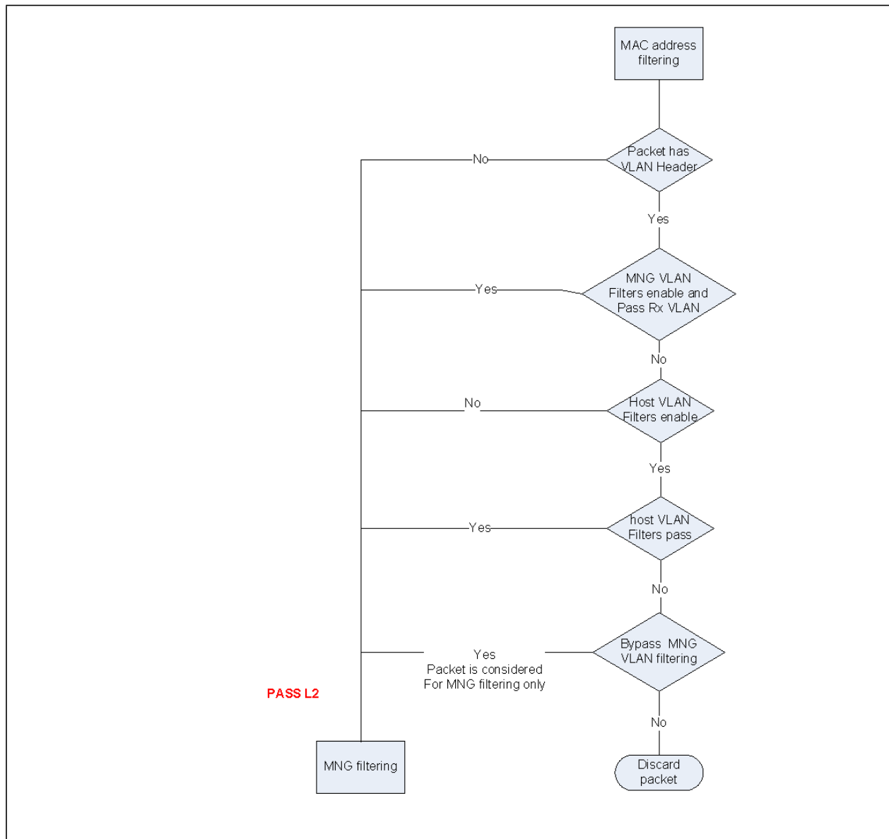
Figure 7-7. VLAN Filtering
