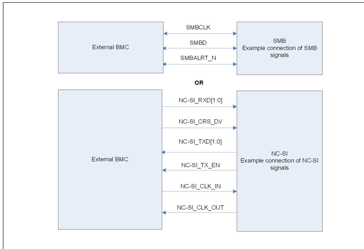
Figure 12-2. External MC Connections with NC-SI and SMB
