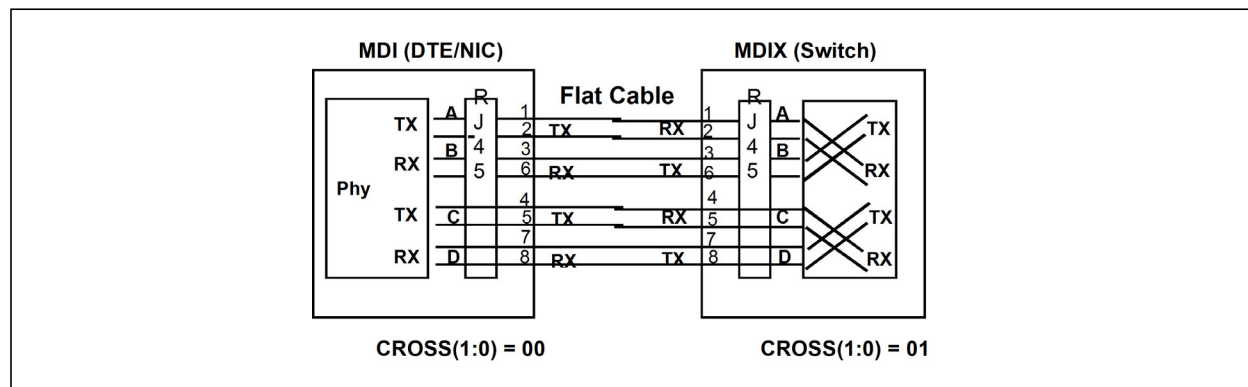
Figure 3-7. Cross-Over Function
