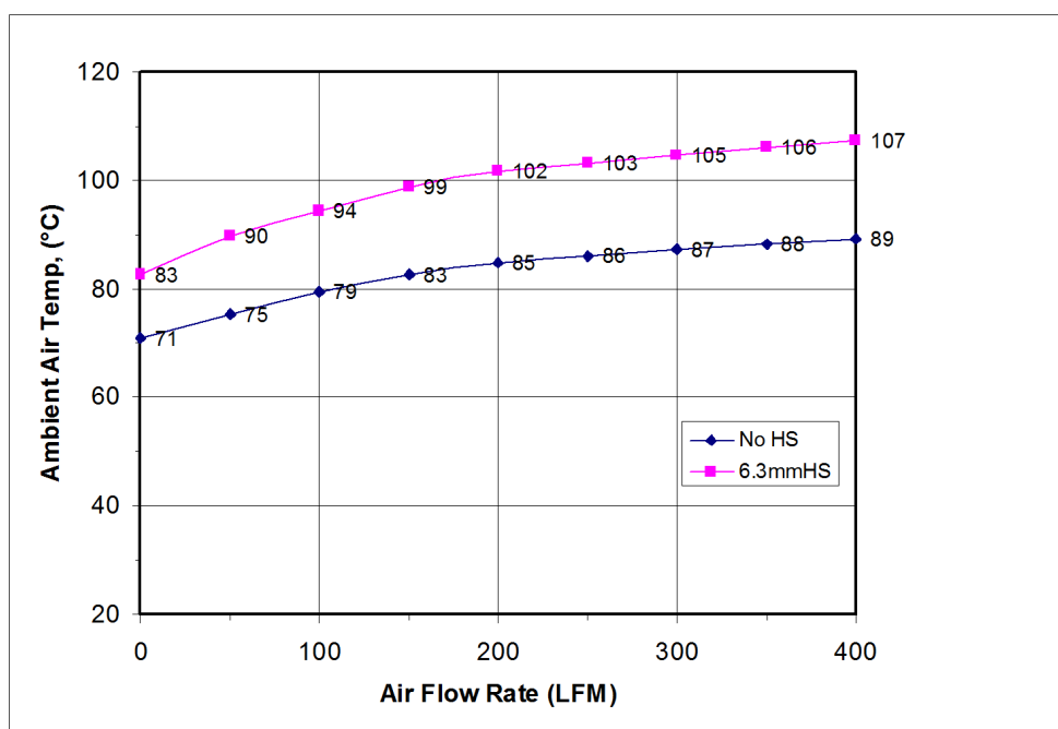
Figure 13-1. Maximum Allowable Ambient Temperature vs. Airflow
