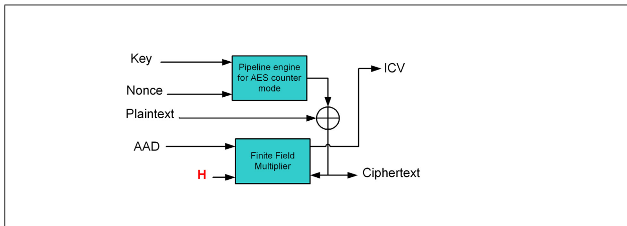
Figure 7-24. AES-128 Crypto Engine Box
