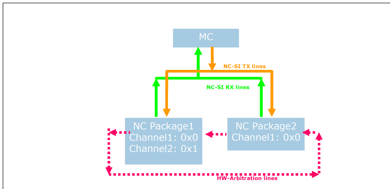
Figure 10-7. Multi-NC Environment
