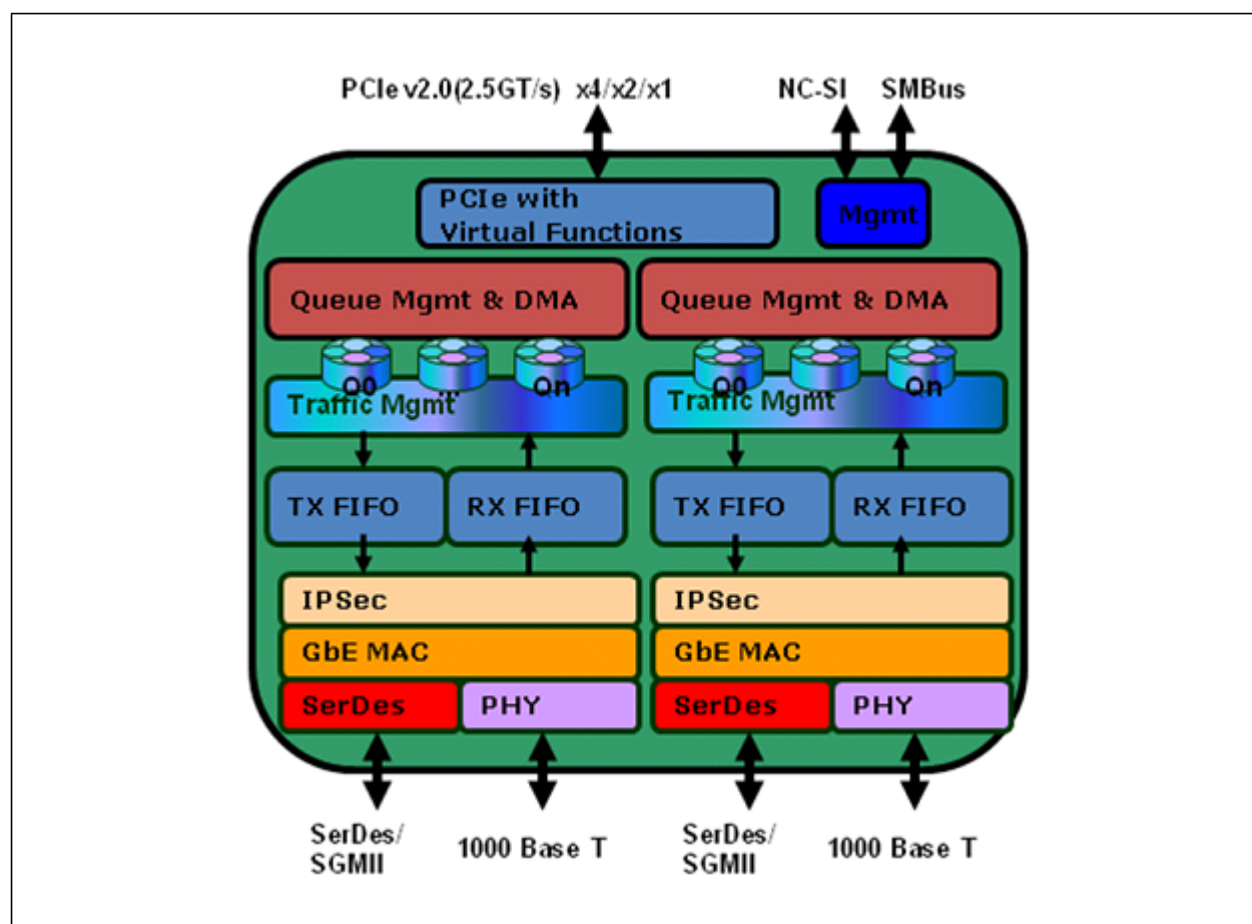
Figure 1-1. 82576 Block Diagram
