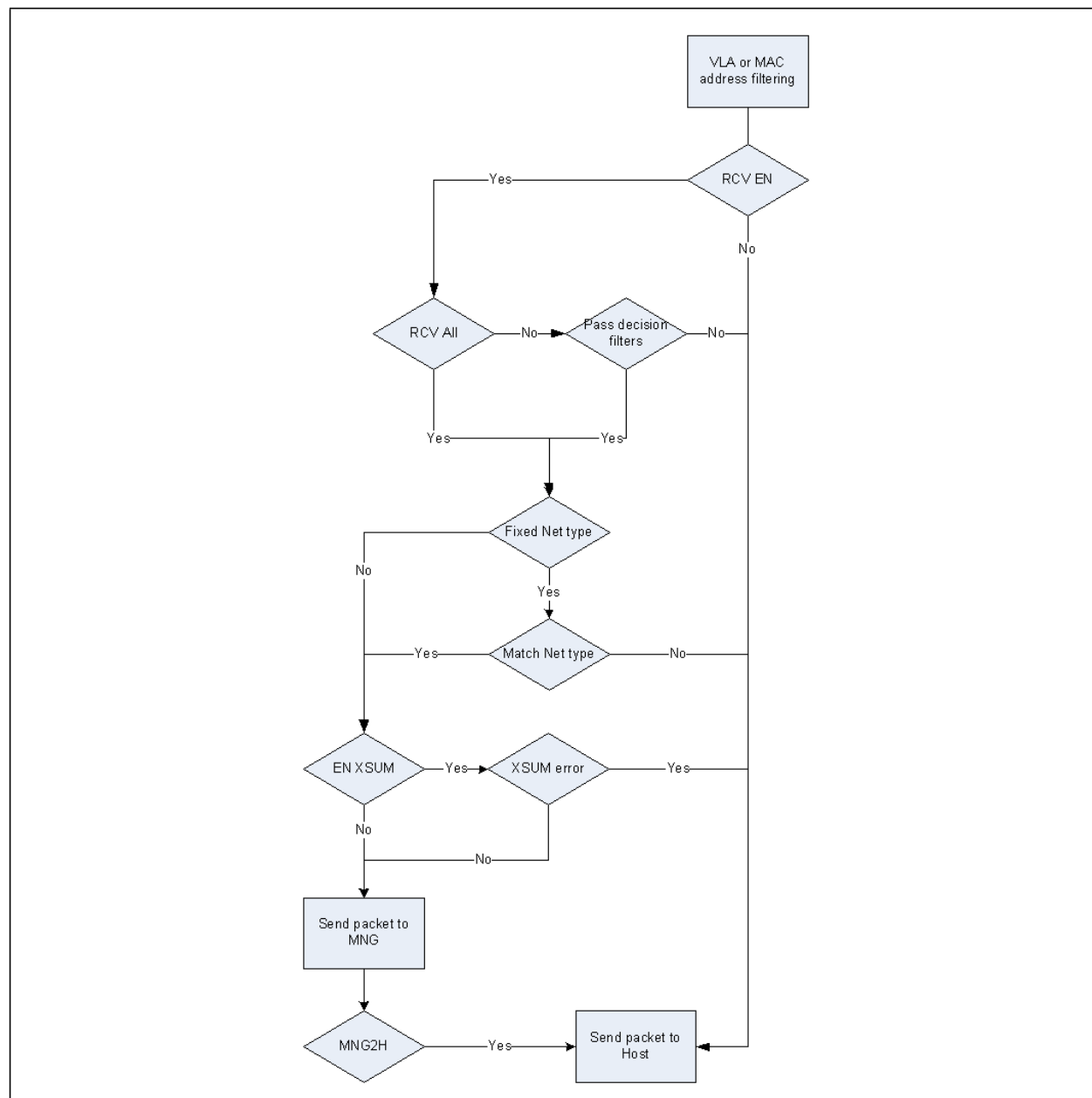
Figure 7-8. Manageability Filtering
