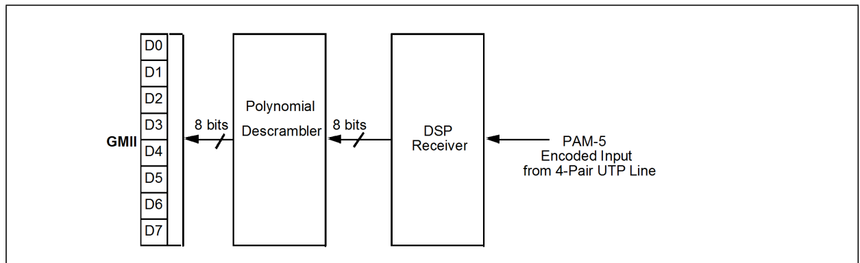
Figure 3-10. Transmit/Receive Flow
