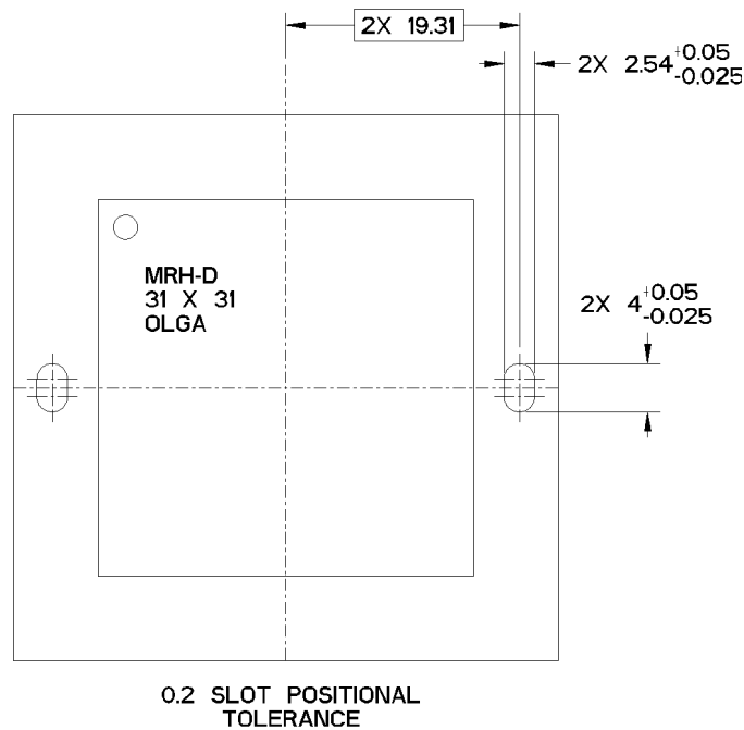
Figure 13-2. 82576EA/EB/ES Heat Sink Volume Restrictions: Primary Side
