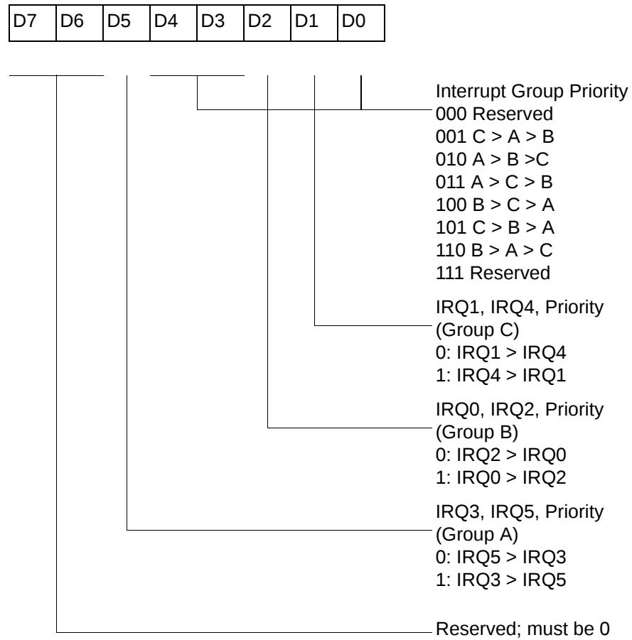
Figure 46. Interrupt Priority Register (F9h: Write Only)
