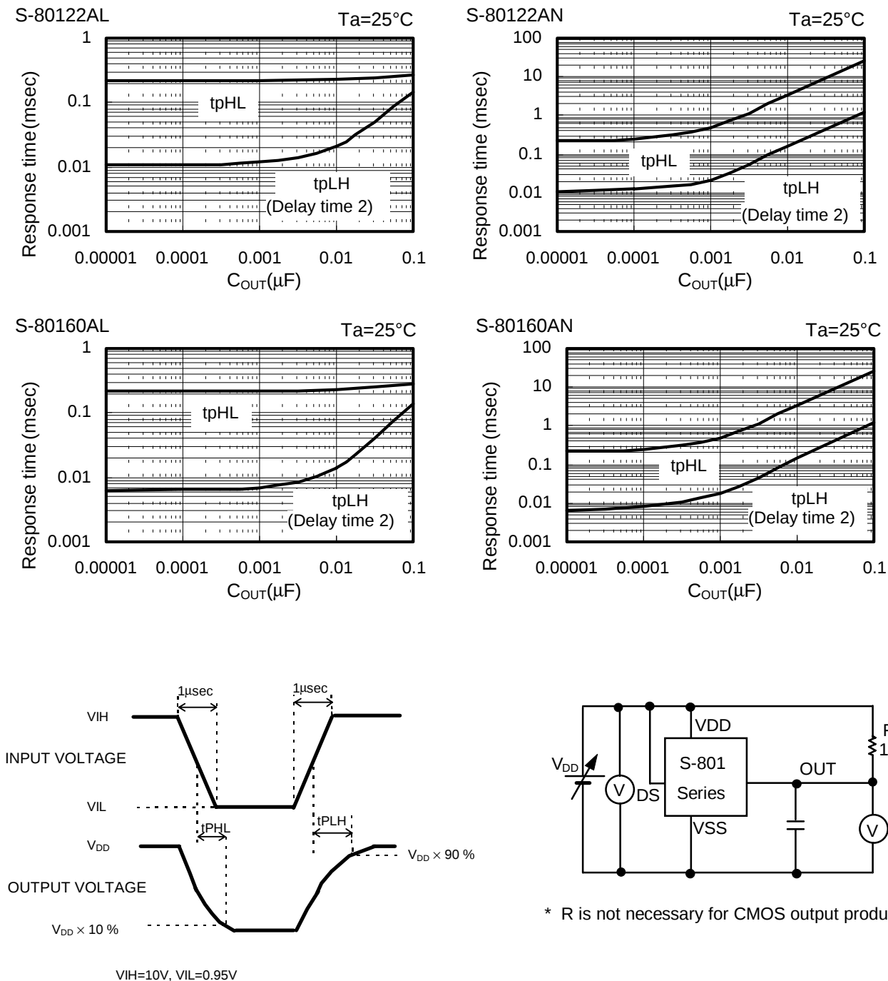
Figure 15 Measuring Conditions of Response Time
