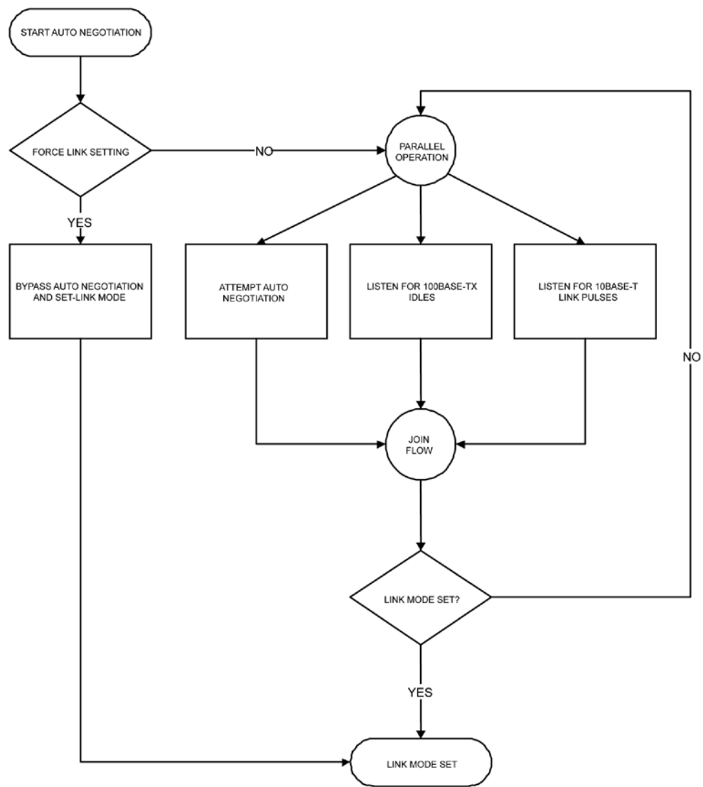
Figure 3. Auto-Negotiation
