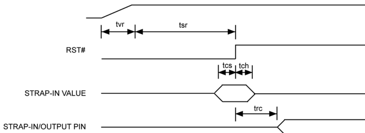
Figure 24. Reset Timing
