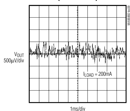
OUTPUT NOISE (10Hz TO 1MHz)
