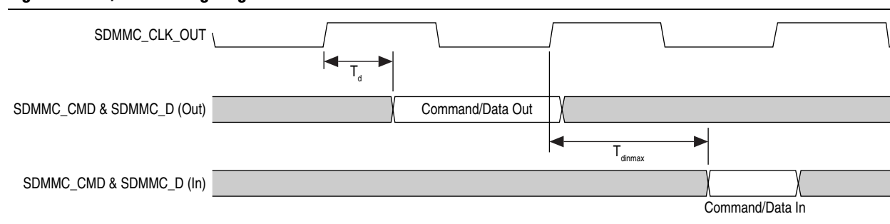
Figure 10. SD/MMC Timing Diagram
