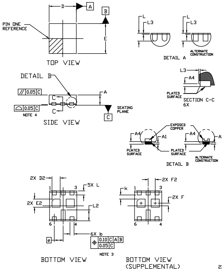
WDFNW6 2.0x2.2, 0.65P CASE 515AK ISSUE A
