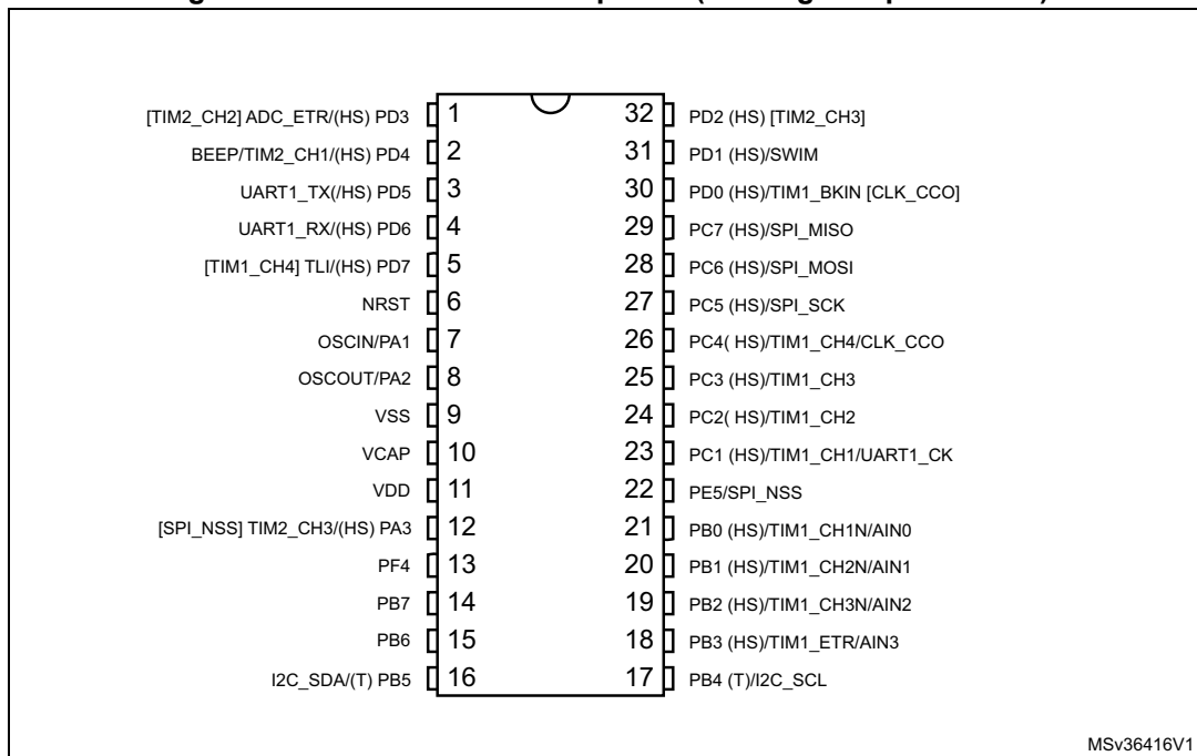
Figure 4. STM8S103K3 SDIP32 pinout (No longer in production)
