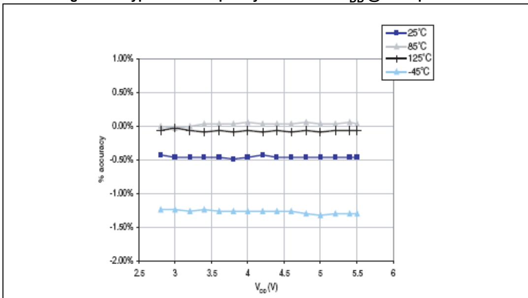
Figure 19. Typical HSI frequency variation vs V_{DD} @ 4 temperatures
