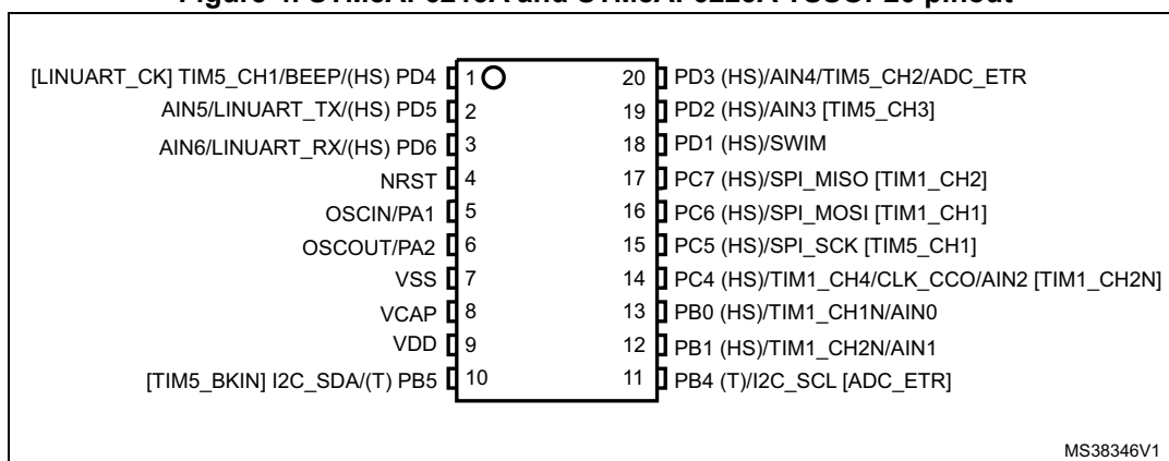
Figure 4. STM8AF6213A and STM8AF6223A TSSOP20 pinout
