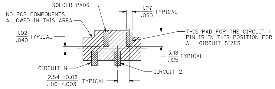
4 CIRCUIT SHOWN
