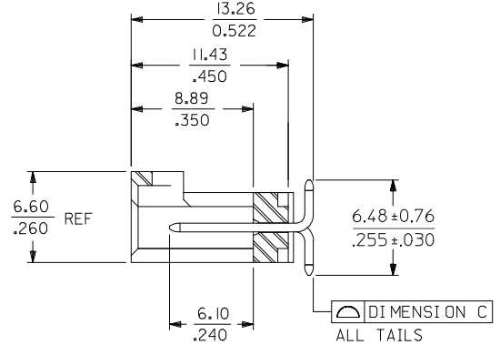
SECTION Z-Z
