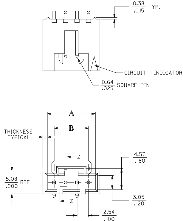
4 CIRCUIT SHOWN
