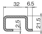
断面拡大図 Cross-section enlarged view
