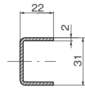
断面拡大図 Cross-section enlarged view
