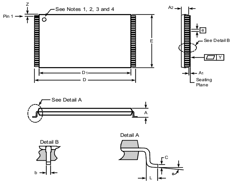
Figure 20. TSOP Package Drawing &amp; Dimensions
