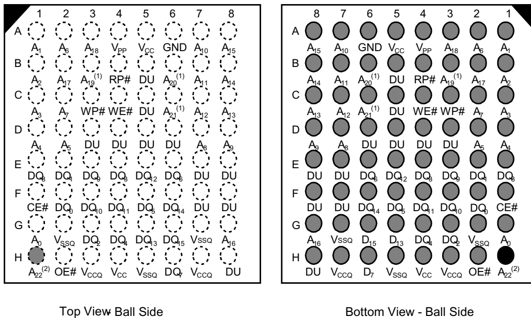
Figure 4. 64-Ball Easy BGA Package 1,2
