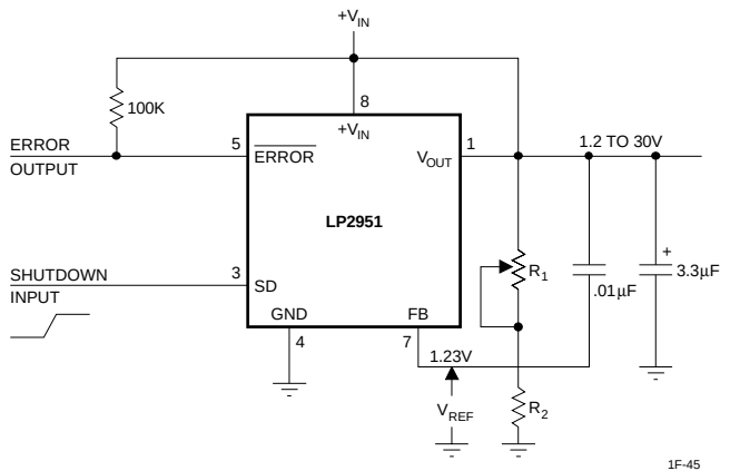
FIGURE 2. ADJUSTABLE REGULATOR
